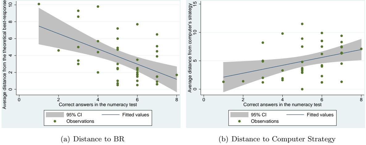
Figure 5: Relationship between the performance in a numeracy test and absolute difference between investments and computer's strategy/best response, averaged by subjects. Incentivized rounds from the second half of the experiment.
