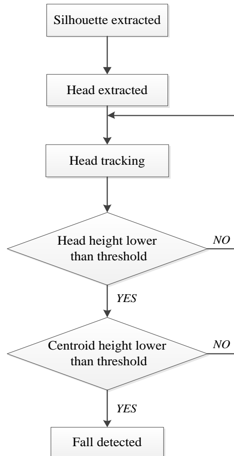
Figure 1. Flow chart of the proposed fall detection method.
