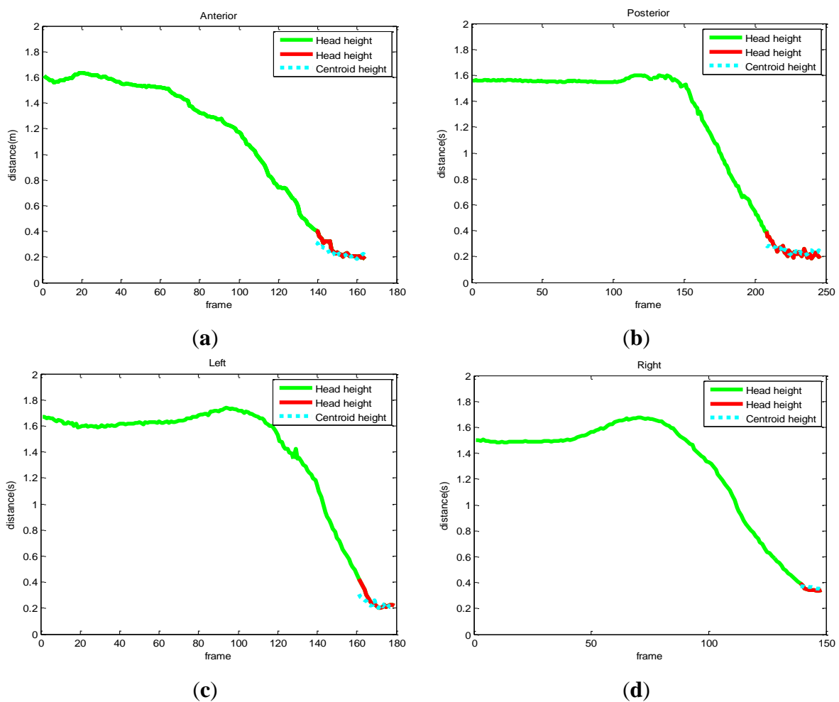
Figure 8. Trajectories of the distance from the head and centroid to the floor in different orientations. (a) Falling down from the anterior orientation; (b) falling down from the posterior orientation; (c) falling down from the left orientation; (d) falling down from the right orientation.
