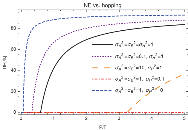
Fig. 3. Relative utility gain between the NE vs. always hopping: D_H = (u^{NE} - u^{Hop,Spread})/u^{NE} as a function of P/\Gamma for N = 32 for different values of \sigma_H^2 , \sigma_A^2 , \sigma_B^2 and \Gamma = 1 .
