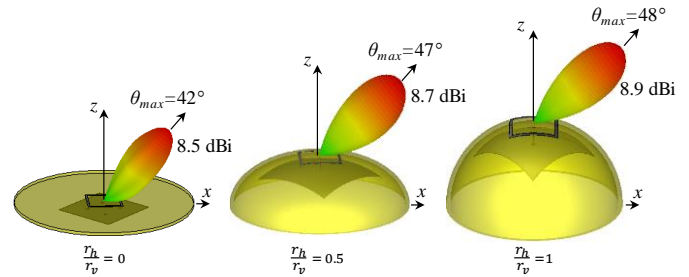
Fig. 5. Effect of substrate bending on the radiation pattern at 2.45 GHz.
