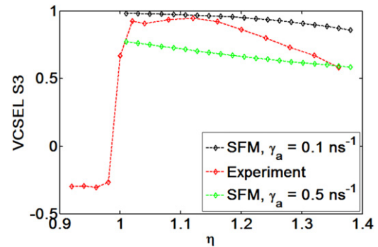
Figure 6. VCSEL ellipticity in the experiment, and in the model for two values of dichroism and fixed pump ellipticity. The sharp change in VCSEL S_3 below threshold in the experiment indicates modal changes, with an associated polarisation change.
