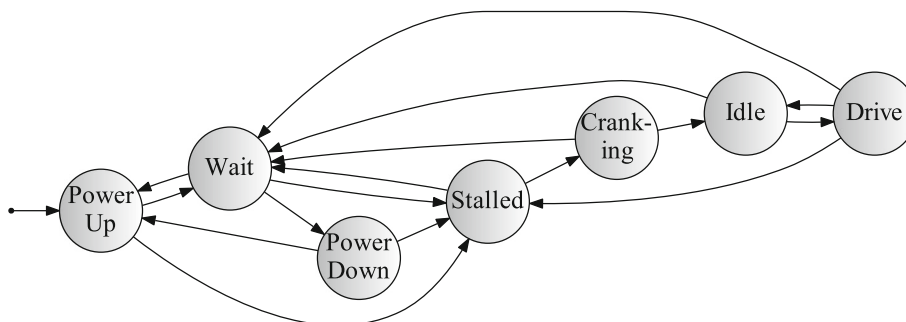
Fig. 2 FSM describing modes in DemoCar
