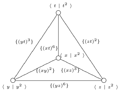
\mathcal{F}_8
