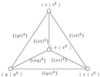
\mathcal{F}_7
