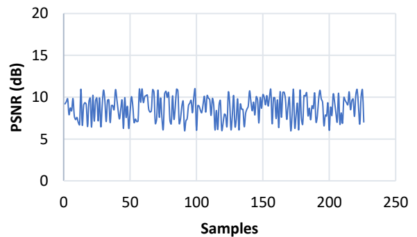
Figure 10: The average values of PSNR for the encrypted and encrypted-watermarked shares for all speech samples.
