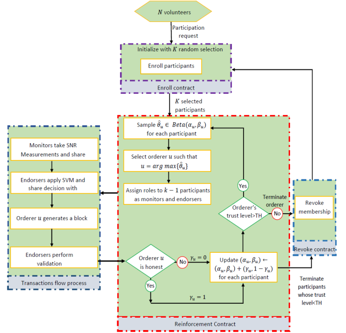
Fig. 4. Flow diagram of the proposed reinforcement learning.
