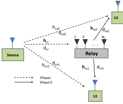
Figure 1: System model with multi-antenna relay and two users.
