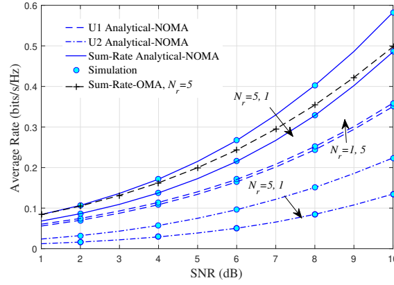
Figure 3: Average rates versus SNR for various values of N_r , when the relay is in AF mode.
