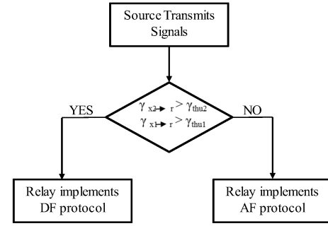
Figure 2: Hybrid relaying protocol.
