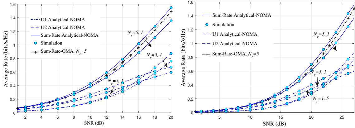
(a) Average rates versus SNR for various values of N_r , when U1 is the strong in the two phases, d_{sr} = 2.5m , d_{su1} = 2m , and d_{su2} = 5m .
