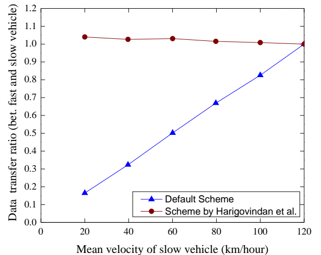
Fig. 2: Data transfer ratio for fast and slow vehicles versus mean velocity of the slow vehicles. Comparison between default DSRC and the scheme proposed by Harigovindan et al. [45].
