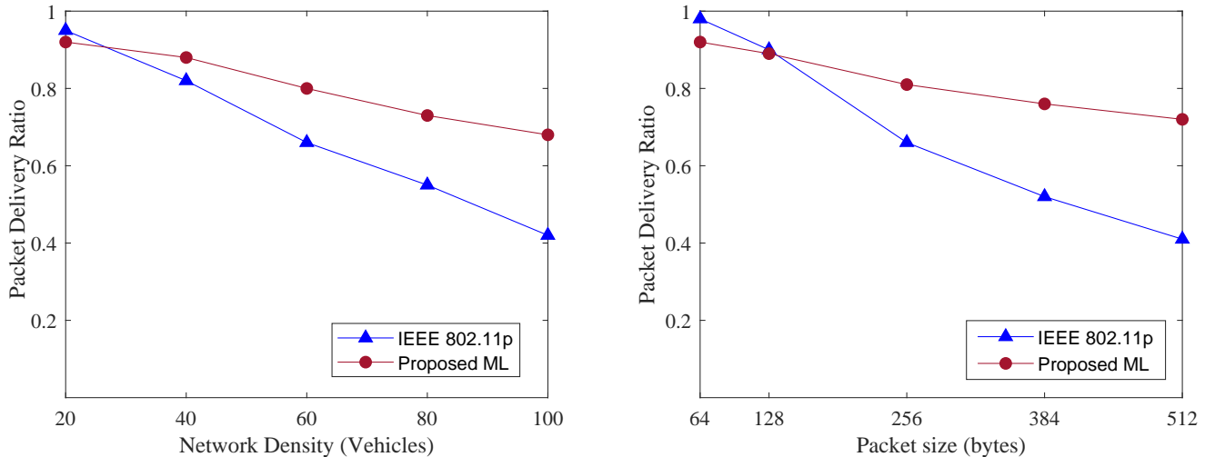
(a) Packet delivery ratio vs. network density for 256 byte packets
