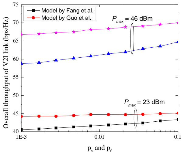
Fig. 10: Throughput comparison between schemes by Guo et al. [85] and Fang et al. [108] with respect to reliability of the V2V link ( p_v ) and cellular user link ( p_f ) [85].
