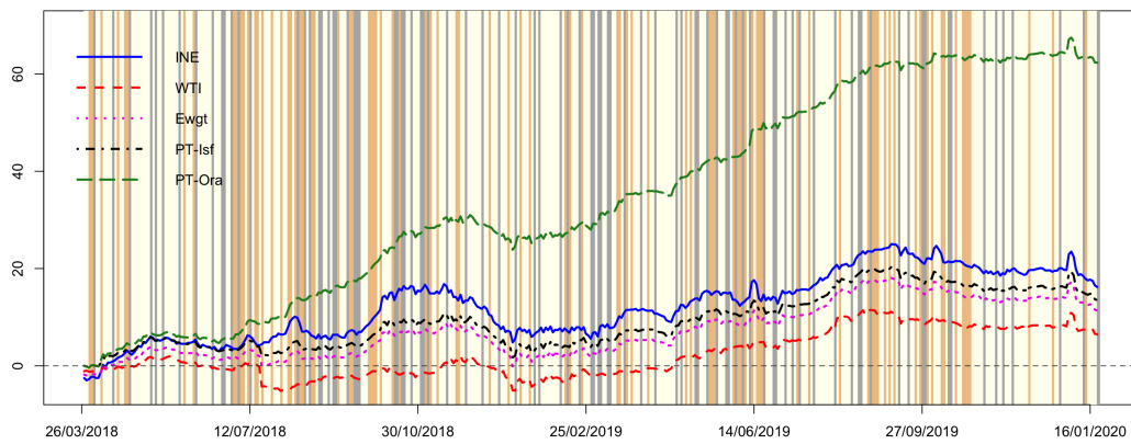
FIGURE 7. The cumulative returns of INE and WTI crude oil futures and their pairs trading strategies in day trading sessions.
