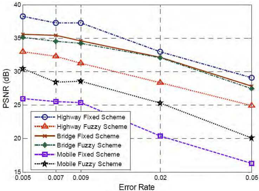
Fig. 17. Video quality according to FLC and equal CBR (fixed) schemes for the ADSL REIN model.
