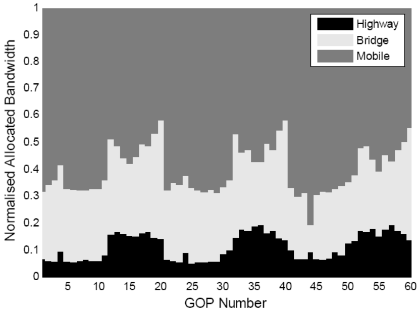
Fig. 14. Bandwidth allocation share per GOP with FLC controller
