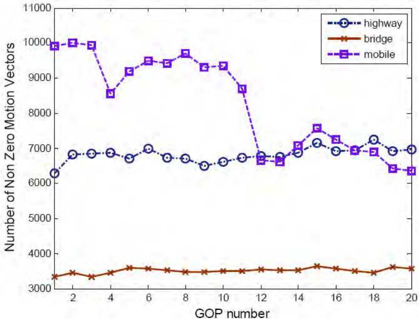
Fig. 11. Number of non-zero motion vectors on a GOP basis
