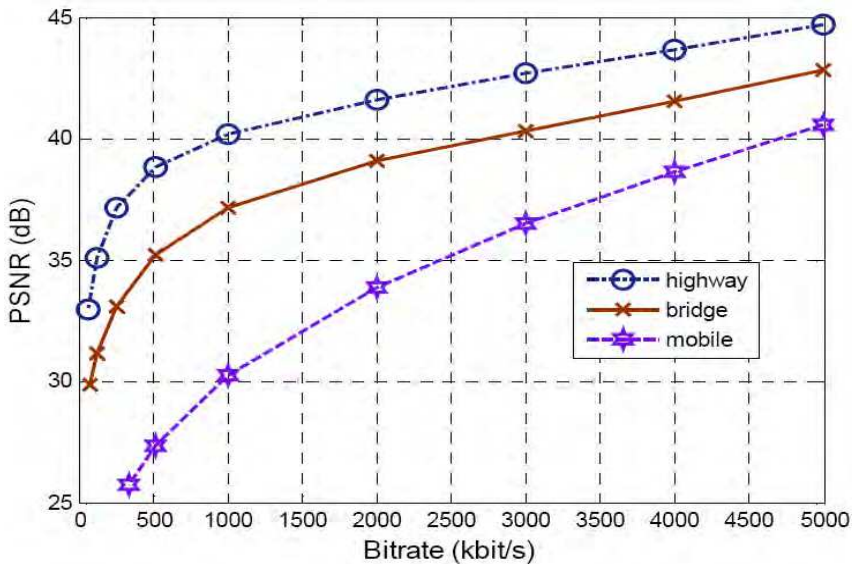
Fig. 9. R-D curves for three well-known video sequences.
