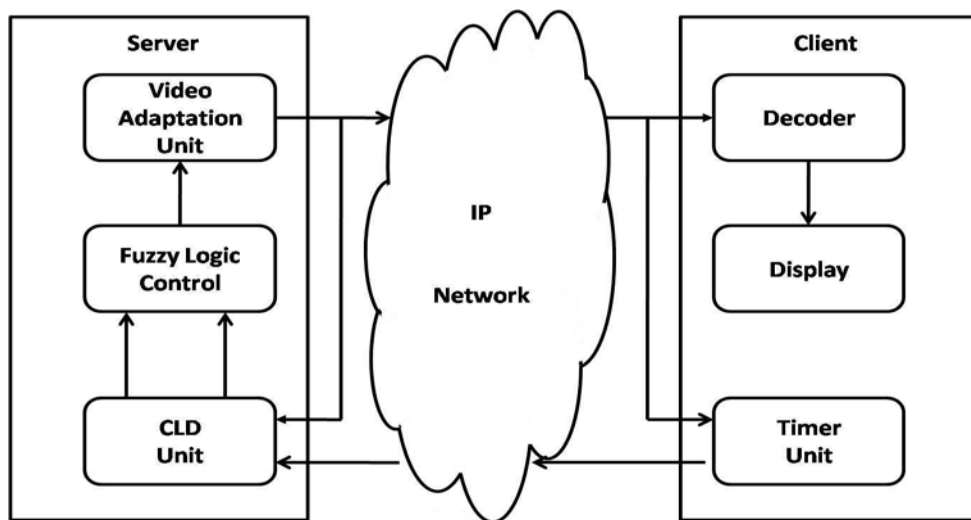
Fig. 5. Video server for all-IP network
