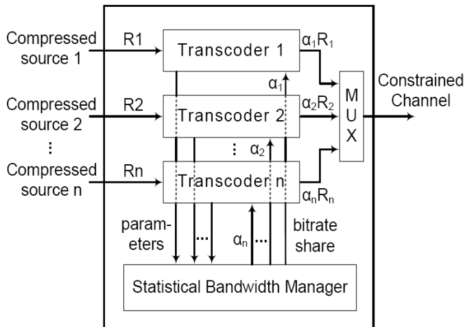
Fig. 10. A statistical multiplexor architecture
