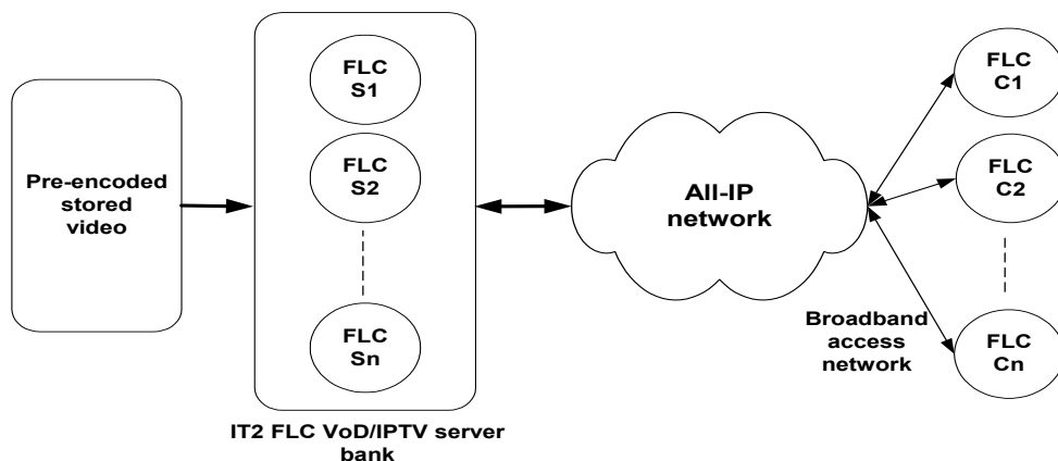
Fig. 6. VoD IPTV video delivery architecture
