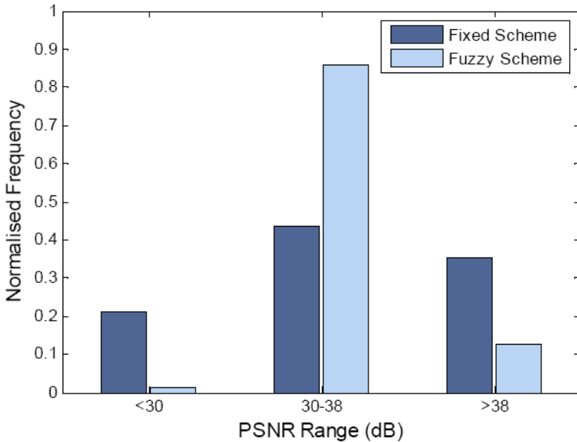
Fig. 15. Normalized per-frame frequencies of video quality for which the three test clips kept within a desired quality range for FLC and equal (fixed) CBR allocation bandwidth
