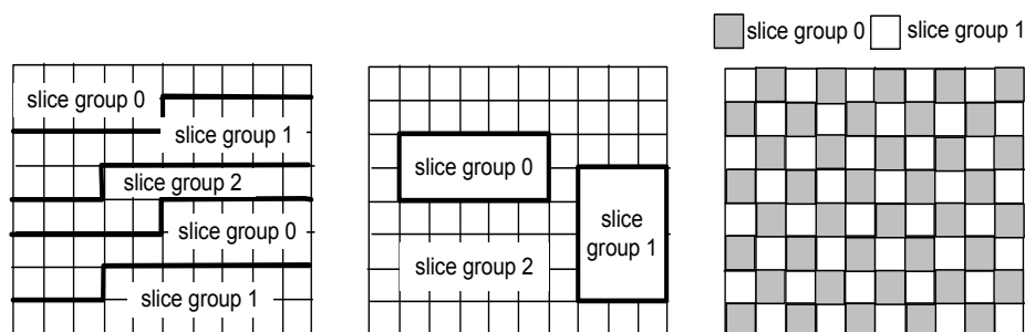
Fig. 1. Example FMO slice groups and types (after (Lambert, 2006) a) Continuing row (type 0) b) geometrical selection (type 2) c) checkerboard selection (type 1)
