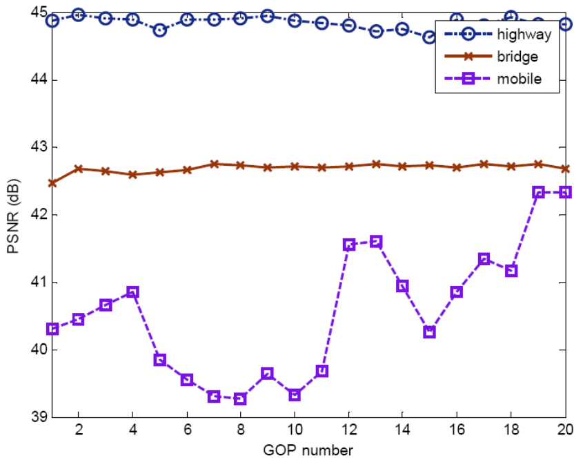
Fig. 13. PSNR fluctuation of input test sequences
