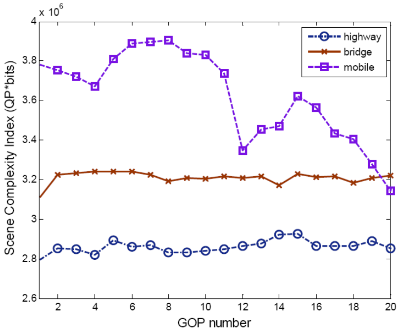
Fig. 12. Scene Complexity Index (SCI) on a GOP basis
