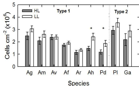
Figure 1: Comparison of symbiont densities across coral species from high and low light growth environments. Type 1 species are Acropora gemmifera (Ag), Acropora microphthalmus (Am), Acropora valiensis (Av), Acropora formosa (Af), Acropora robusta (Ar) Acropora horrida (Ah), and Pocillopora damicornis (Pd);
