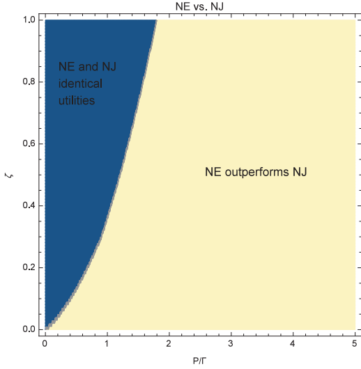
Fig. 2. NE vs. NJ regions as functions of P/\Gamma \geq 0 and 0 \leq \zeta \leq 1 for \sigma^2 = \sigma_H^2 = 1 .
