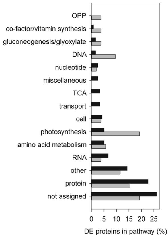
Fig. 4. Functional classification of differentially expressed (DE) proteins in low- \text{CO}_2 -adapted pyr+ (black) and pyr- (grey) cells.
