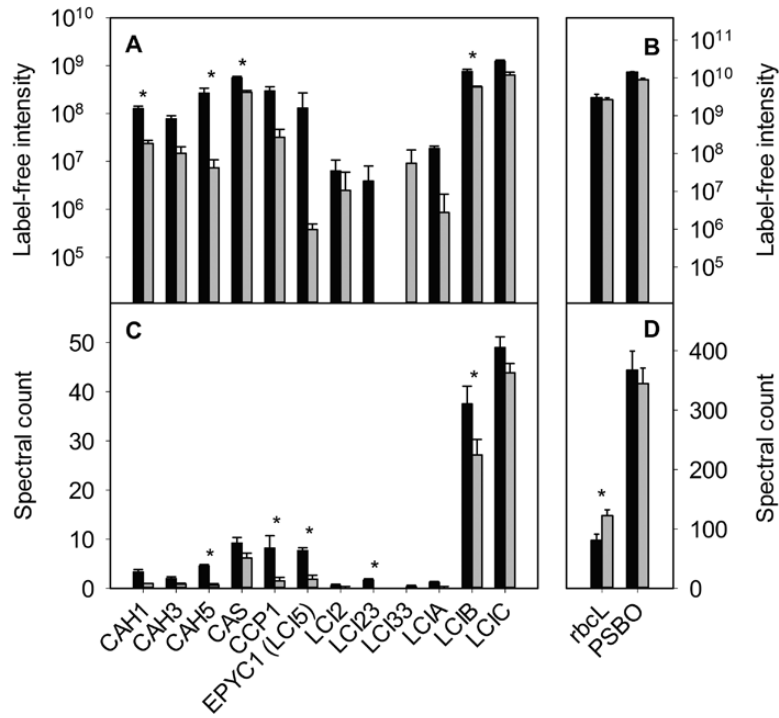
Fig. 3. Relative quantification of 12 CCM proteins detected in low- \text{CO}_2 -adapted pyr+ (black) and pyr- (grey) strains using LC-MS/MS. CCM and \text{CO}_2 -responsive proteins (A, C), non- \text{CO}_2 -responsive ( rbcL ), and photosynthetic/control (PSBO) proteins (B, D) are shown. Note the different scales of the y-axes. Two measures of protein abundance were used: label-free (ion) intensity, which is proportional to absolute abundance (A, B), and spectral count, which is a measure of the relative abundance in the sample (C, D). Values shown are the mean and standard error of six measurements (two technical replicates for three replicate cultures). Asterisks represent statistically significant differences ( P < 0.05 ) in protein abundance between the two strains according to a t -test on label-free intensity values or a G-test on spectral counts.
