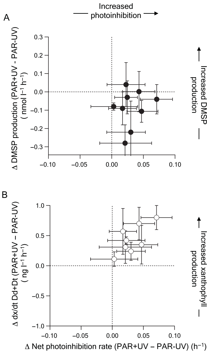
Fig. 7. Physiological response to irradiance-mediated photoinhibition in phytoplankton communities of the northeastern Tropical Atlantic. (A) Difference in DMSP production ( \Delta DMSP production) related to differences in photoinhibition ( \Delta net photoinhibition rate) between incubation treatments (PAR+UV – PAR-UV). DMSP production was calculated from \mu DMSP and initial DMSP concentration. (B) Difference in xanthophyll pigment production ( \Delta dx/dt Dd + Dt) and \Delta net photoinhibition rate between incubation treatments (PAR+UV – PAR-UV). \Delta DMSP production and \Delta dx/dt Dd + Dt were calculated over the time intervals prior to the point of maximum photoinhibition (Fig. 3). Error bars are the propagated SD.
