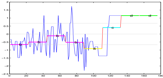
Figure 7: A real time average speed data obtained from a pair of sensor points given in Figure 6 is mapped into SAX word, "bbbbacdd", with the segment size of "8" and alphabet size of "4" for 176 samples.
