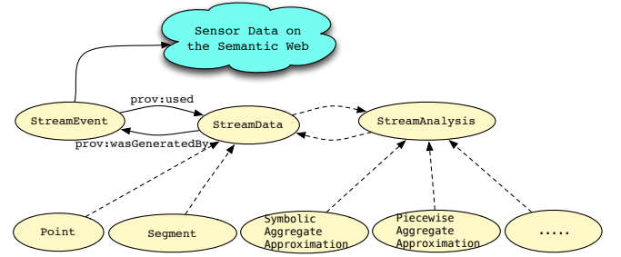
Figure 4: Depiction of the main concepts and relationships in the Stream Annotation Ontology.
