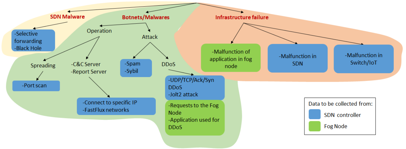
Fig. 1. Taxonomy of attacks endangering an IoT network
