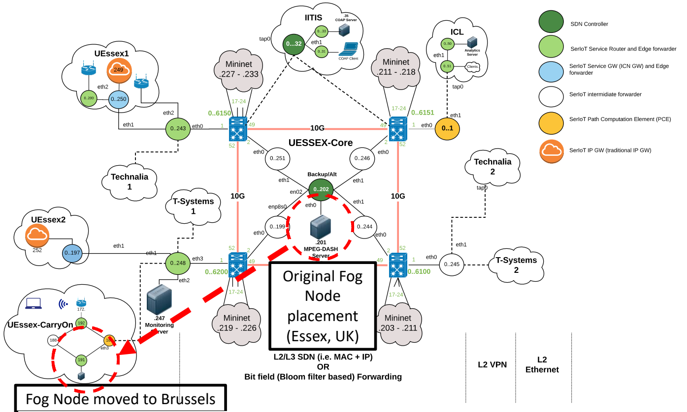
Fig. 3. Demonstration of moving a Fog Node dynamically in the SerIoT testbed, demonstrating reduced service latency
