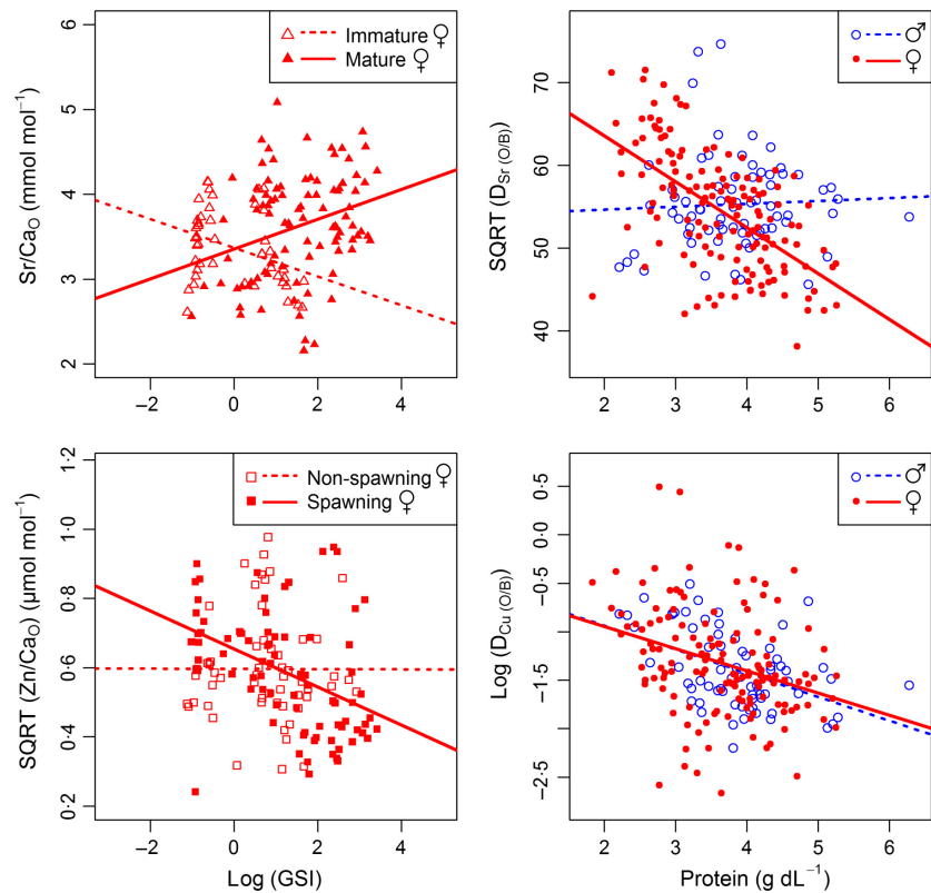
Fig. 6. The strongest relationships between gonadosomatic index (GSI) and otolith element/calcium ratios ( \text{El}/\text{CaO} ) in mature vs. immature and spawning vs. non-spawning female plaice, and between blood plasma-otolith distribution coefficients ( D_{\text{El}(\text{O/B})} ) and plasma protein concentrations of male ( \sigma ) and female ( \varphi ) plaice serially sampled for 7–12 months. Some variables were transformed to meet model assumptions of homogeneity and normally distributed residuals.
