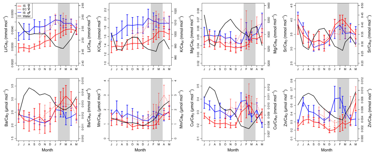
Fig. 4. Average ( \pm SE) otolith element/calcium ratios (El/CaO) in 19 plaice from the Irish Sea (IS) and English Channel (EC) serially sampled for 7–12 months. Note that sampling was carried out twice in February. Shading = peak spawning period. ♀ = female, ♂ = male.
