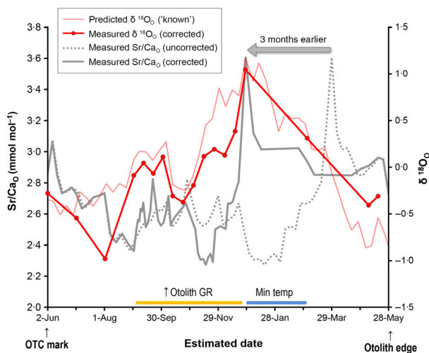
Fig. 2. Predicted otolith \delta^{18}\text{O} values ( \delta^{18}\text{O}_{\text{OTC}} ) based on measured temperature and salinity were used to temporally match measured \delta^{18}\text{O}_{\text{OTC}} values and otolith elemental ratios such as \text{Sr}/\text{Ca}_{\text{OTC}} . The otolith presented here exhibited elevated growth rates (GR) during the first half of the study (orange bar), prior to spawning and the period of thermal minima (blue bar). Temporal corrections resulted in the maximum \text{Sr}/\text{Ca}_{\text{OTC}} value being assigned a calendar date 3 months earlier than would have been estimated had constant growth rates been assumed.
