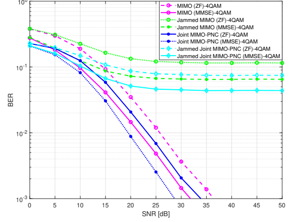
Fig. 3. BER performance comparison between i) conventional multi-user MIMO ii) multi-user MIMO with jamming, iii) multi-user MIMO with PNC and iv) multi-user MIMO with PNC and jamming, with 10dB jamming SJR, for M=4 , N=2 , K=2 and J=2 .
