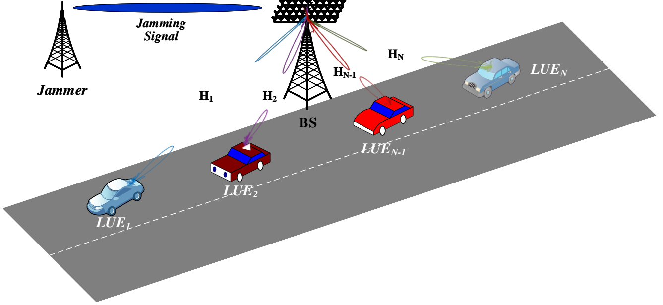
Fig. 1. A System Model for a Multi-user Massive MIMO Vehicular Network under Jamming Attack.
