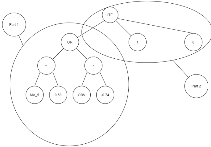
Fig. 1. Example of the GP tree structure and the If-then-else structure
