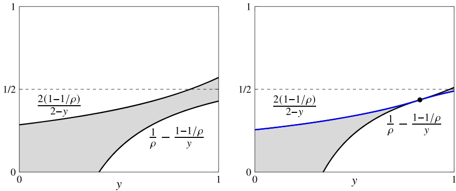
Fig. 2 Pictorial views of the statement of Lemma 5 for \rho = 7/5 (left) and \rho = 7 - 4\sqrt{2} (right). The gray area corresponds to the available space that allows for the definition of (the function c of) expert-independent mechanisms with approximation ratio at most \rho . The truthfulness requirements are obtained if c is non-decreasing (for BCh-IC; see Lemma 1) and takes values not higher than 1/2 (for BSw-IC; see Lemma 6). The blue line at the right is the c -function used by our mechanism EIM, which has all the above properties for \rho = 7 - 4\sqrt{2} (color figure online)
