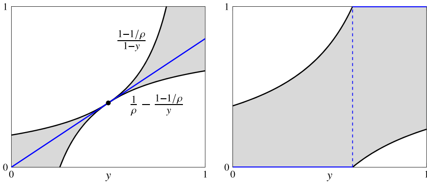
Fig. 3 Pictorial views of the statement in Lemma 8 for \rho = 5/4 (left) and \rho = \phi (right). The gray area in both plots corresponds to the available space for the definition of \mathcal{T} mechanisms (e.g., mechanisms R and D which are depicted by the blue lines) (color figure online)
