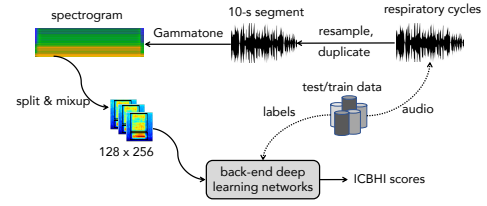
Fig. 1. Deep learning based framework proposed
