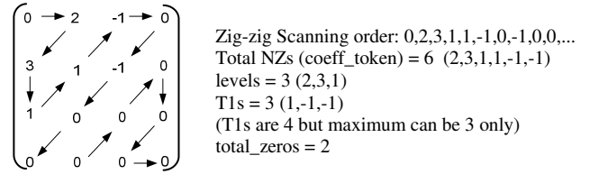
Fig. 1. Illustrative example of 4x4 sub-macroblock coefficients coded by VLC
