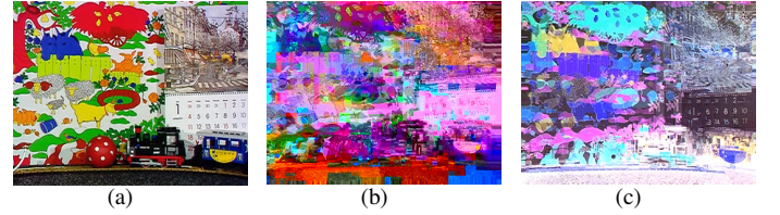
Figure 3. Impact of selective encryption on the PSNR of Mobile (CIF) sequence encoded with 300 frames (I+P+B) and QP 18. (a) Frame # 156 [Y=38.9, U=41.5, V=41.4 dB]. (b) Proposed SE on CAVLC [Y=12.6, U=13.2, V=11.3 dB]. (c) Proposed SE on CABAC [Y=6.9, U=12.6, V=13.3 dB].
