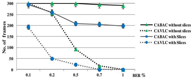
Figure 6. The mean number of frames decoded after a bit-error in the Foreman sequence when using the CABAC or CAVLC entropy coders (error bars show one standard deviation).
