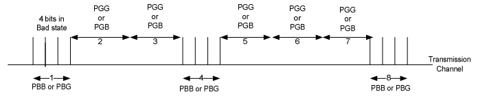
Fig. 2. G-E model state transitions over a transmission channel
