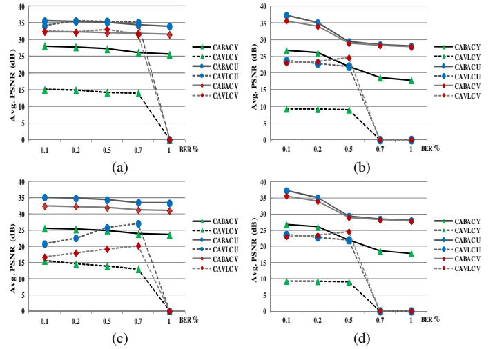
Figure 5. Impact of bit-errors on PSNR of test sequences with varying BER. (a) Foreman average PSNR of CABAC and CAVLC encoded bit-streams without slices. (b) Foreman average PSNR of CABAC and CAVLC encoded bit-streams with slices. (c) Mobile average PSNR of CABAC and CAVLC encoded bit-streams without slices. (d) Mobile average PSNR of CABAC and CAVLC encoded bit-streams with slices.
