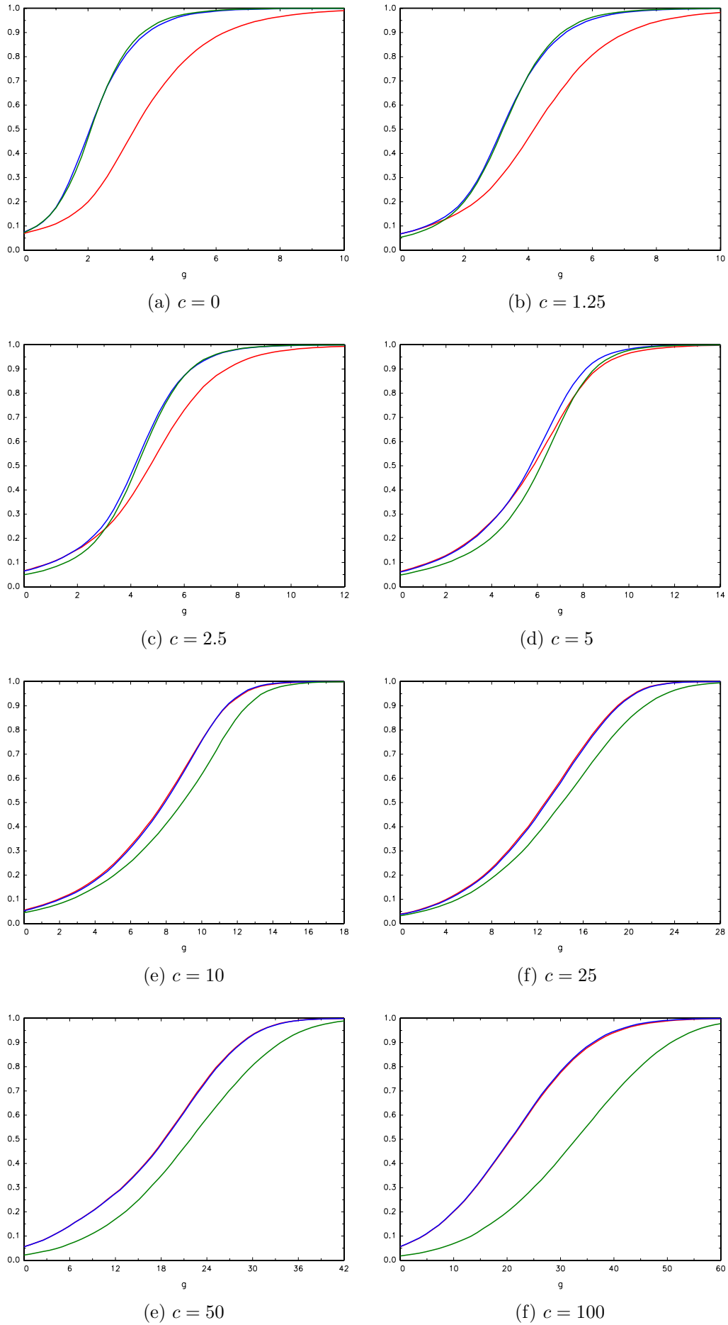
Figure 5. Finite sample power of nominal 0.05-level tests, T = 200 , \rho_{xy} = -0.95 ; \mathcal{T}_{hyb} : —, \mathcal{T}_{hyb}^w : —, EMW : —
