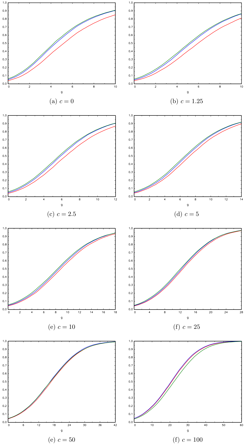
Figure 8. Finite sample power of nominal 0.05-level tests, T = 200 , \rho_{xy} = -0.1 ; \mathcal{T}_{hyb} : —, \mathcal{T}_{hyb}^w : —, EMW : —
