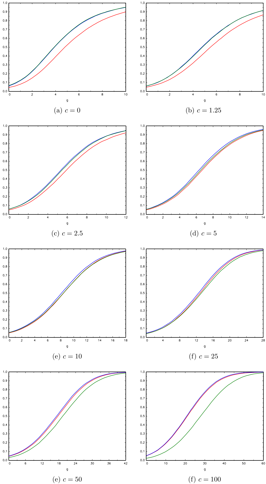
Figure 7. Finite sample power of nominal 0.05-level tests, T = 200 , \rho_{xy} = -0.5 ; \mathcal{T}_{hyb} : —, \mathcal{T}_{hyb}^w : —, EMW : —
