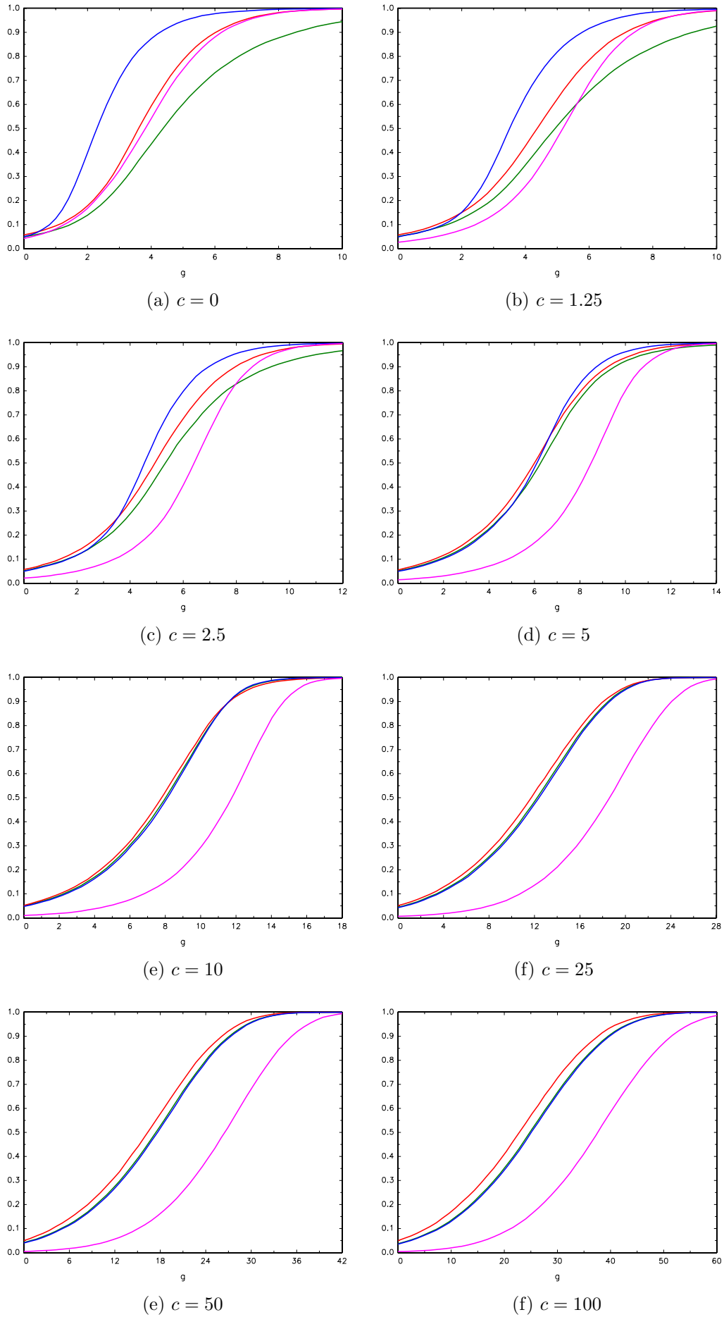
Figure 1. Asymptotic local power of nominal 0.05-level tests, \rho_{xy} = -0.95 ; \mathcal{T}_{con}^* : —, \mathcal{T}'_{con} : —, \mathcal{T}_{con} : —, \mathcal{T}_{con}^w : —
