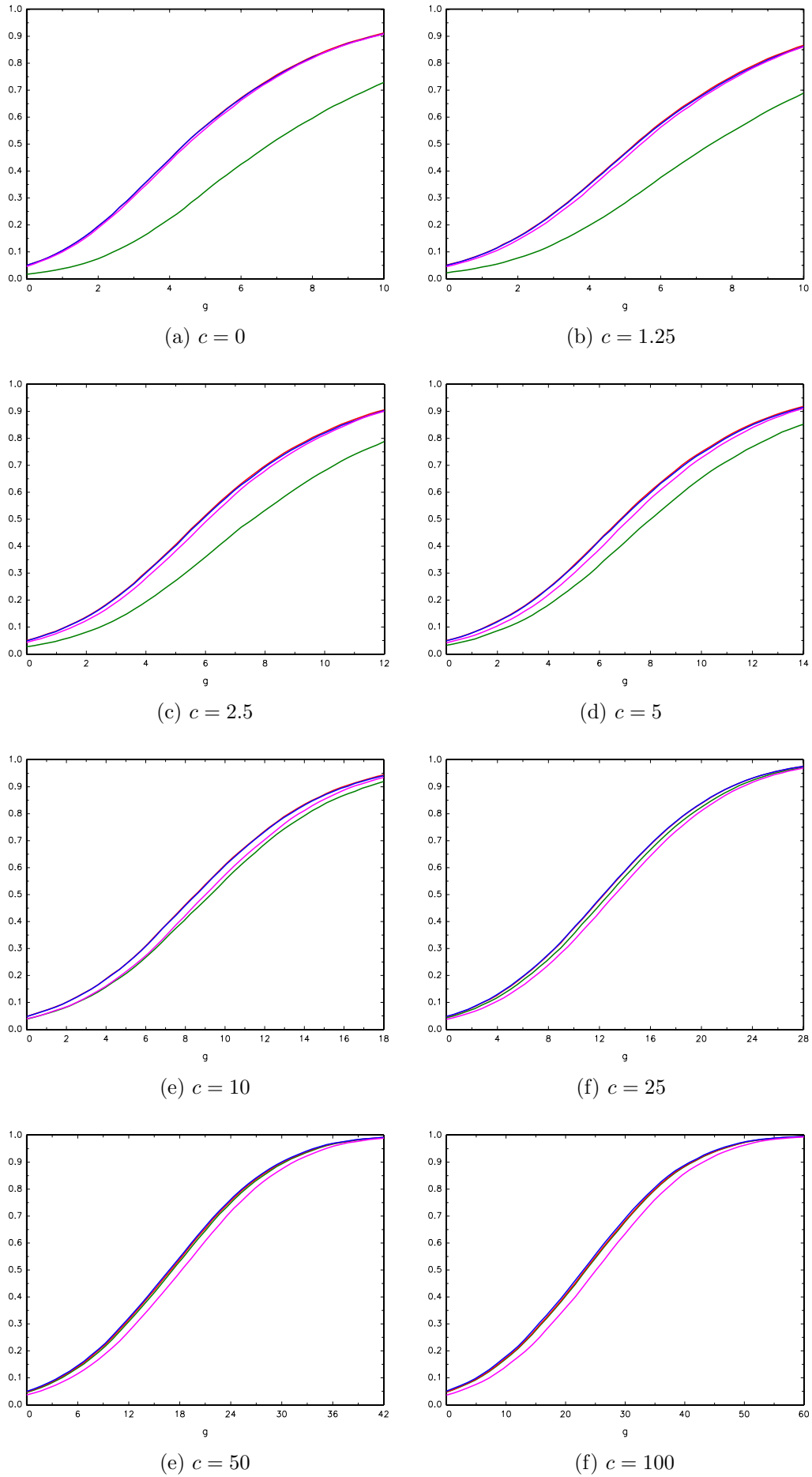
Figure 4. Asymptotic local power of nominal 0.05-level tests, \rho_{xy} = -0.1 ; \mathcal{T}_{con}^* : —, \mathcal{T}'_{con} : —, \mathcal{T}_{con} : —, \mathcal{T}_{con}^w : —
