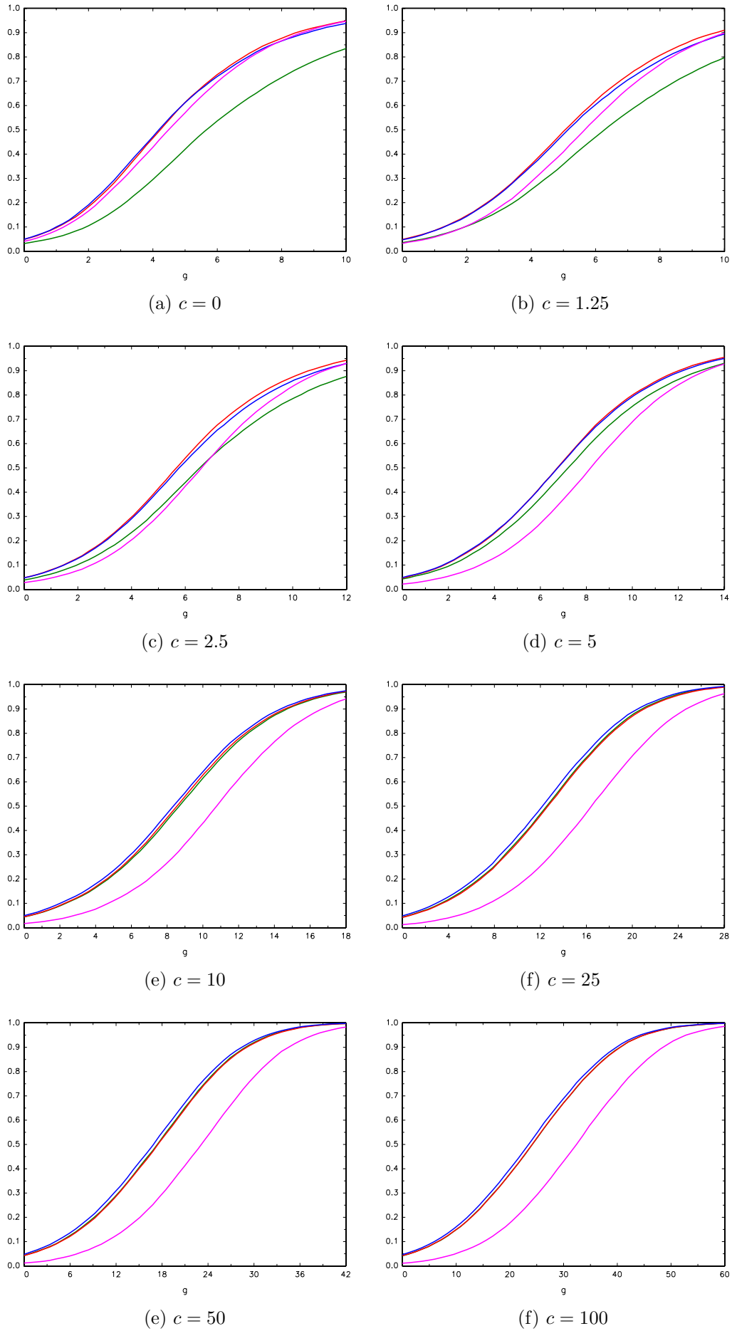
Figure 3. Asymptotic local power of nominal 0.05-level tests, \rho_{xy} = -0.5 ; \mathcal{T}_{con}^* : —, \mathcal{T}'_{con} : —, \mathcal{T}_{con} : —, \mathcal{T}_{con}^w : —
