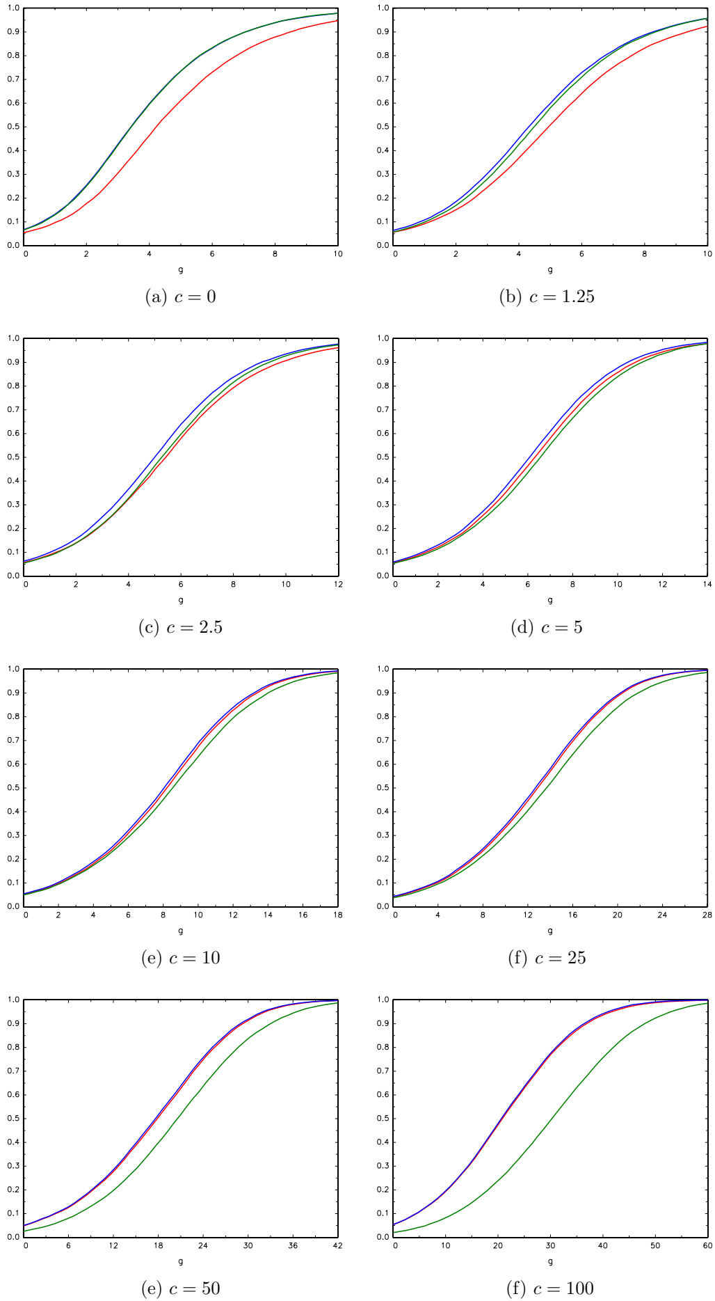
Figure 6. Finite sample power of nominal 0.05-level tests, T = 200 , \rho_{xy} = -0.7 ; \mathcal{T}_{hyb} : —, \mathcal{T}_{hyb}^w : —, EMW : —
