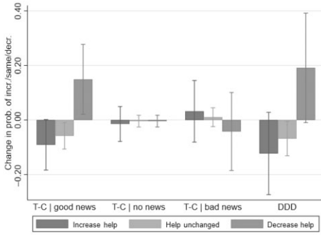
(a) AR(1)
