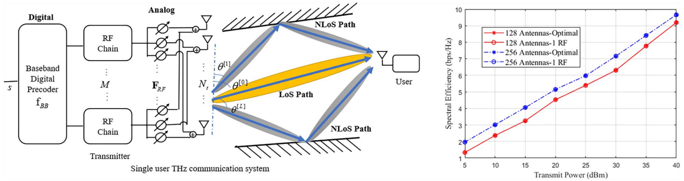
FIGURE 2 Spectral efficiency in single user communication system.
