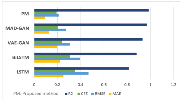
Fig. 3. Graphical representation of performance evaluation metrics for various state-of-art techniques for anomaly detection
