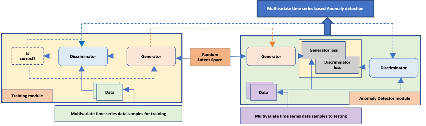
Fig. 1. Pictorial illustration of the proposed model (CNN-BiLSTM GAN)
