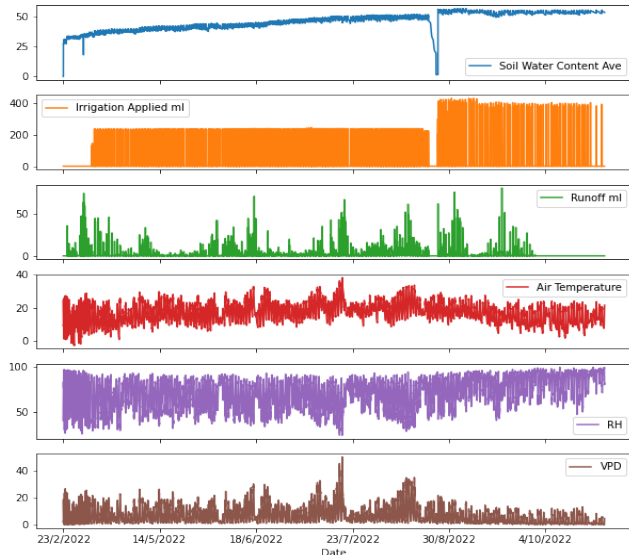
Fig. 2. Historical trend various sensors on a system for a cherry garden
