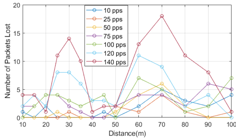
Figure 8. Packets lost over distance.
