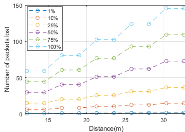
Figure 15. Percentage of consecutive packet loss.
