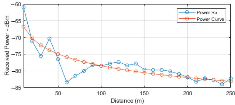
Figure 7. Receiver power over distance.
