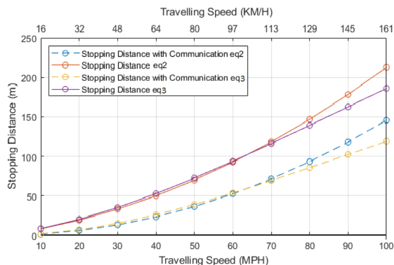
Figure 2. Stopping distance comparison.
