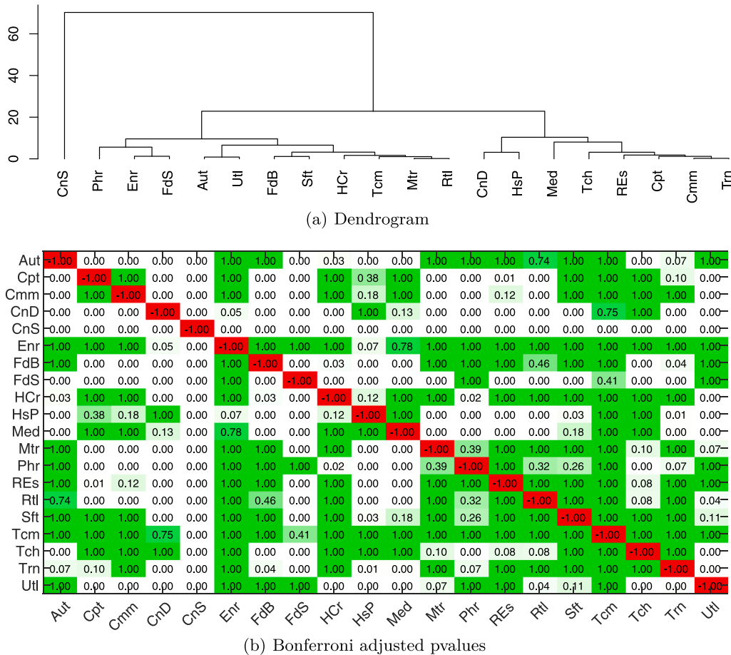
Fig. 1. Top: A dendrogram of the cluster of sector effects of the change in MORE ratings between 2019–2020, using the ANCOVA model. Bottom: The matrix of Bonferroni adjusted p-value for pairwise t-test between means of the sectors, using the ANCOVA model. The off-diagonals are color-coded to describe the sign of the statistical relationships, with green signifying difference in means (i.e. p\text{-value} > 0.05 ), and white for non-significant differences.
