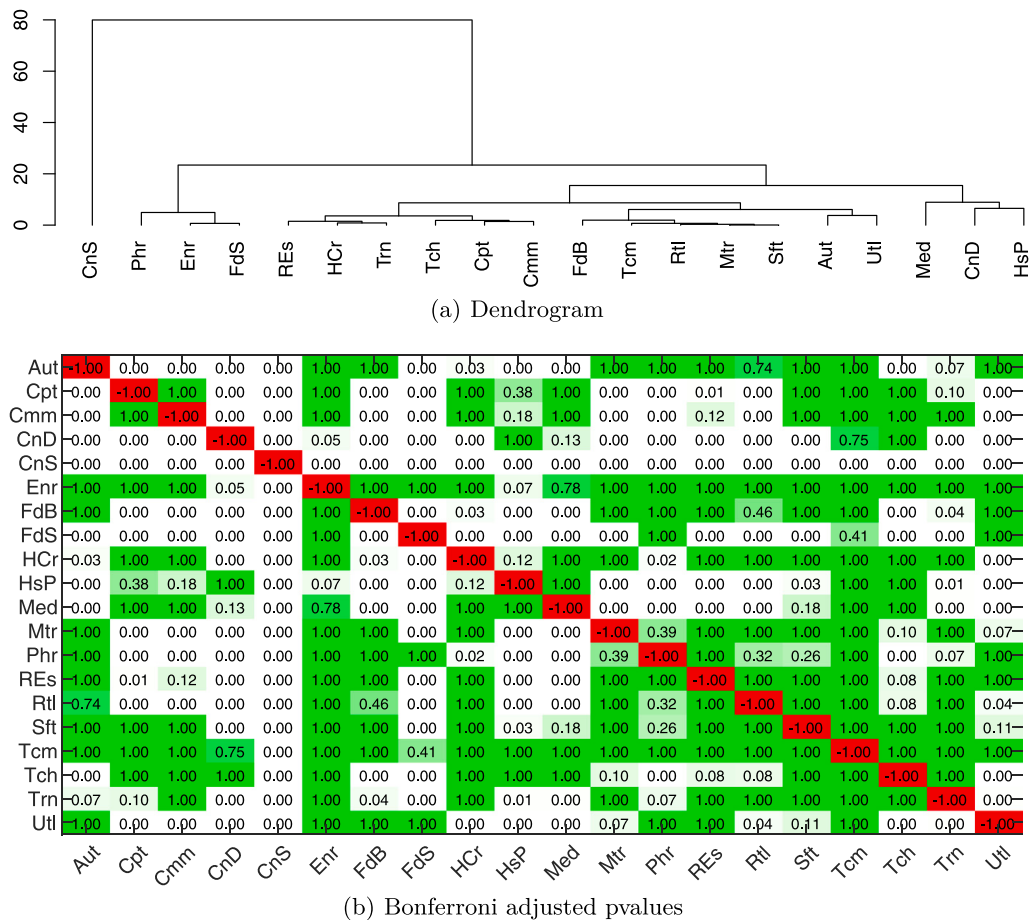
Fig. 2. Top: A dendrogram of the cluster of sector effects of the change in MORE ratings between 2019–2020, using the ANCOVA-ARDL model. Bottom: The matrix of Bonferroni adjusted p-value for pairwise t-test between means of the sectors, using the ANCOVA-ARDL model. The off-diagonals are color-coded to describe the sign of the statistical relationships with green signifying difference in means (i.e. p-value > 0.05), and white for non-significant differences.
