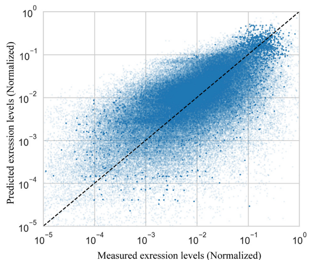
FIGURE 7 Comparison between measured expression levels of 2851 genes for 217 transcription records and gene expression values computed by the extracted full GRNN.
