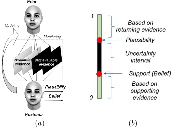
Fig. 6. The DS uncertainty interval. The DS technique can handle uncertainty, or ignorance, ythat is, lack of knowledge of the complete probabilistic model required for Bayesian inference.
