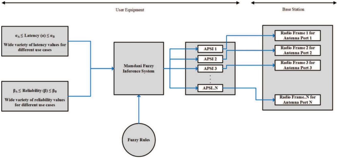
Fig. 1: System Model for obtaining Dynamic Radio Frame Configuration from APSI transmitted by UE in the uplink via physical uplink control channel.
