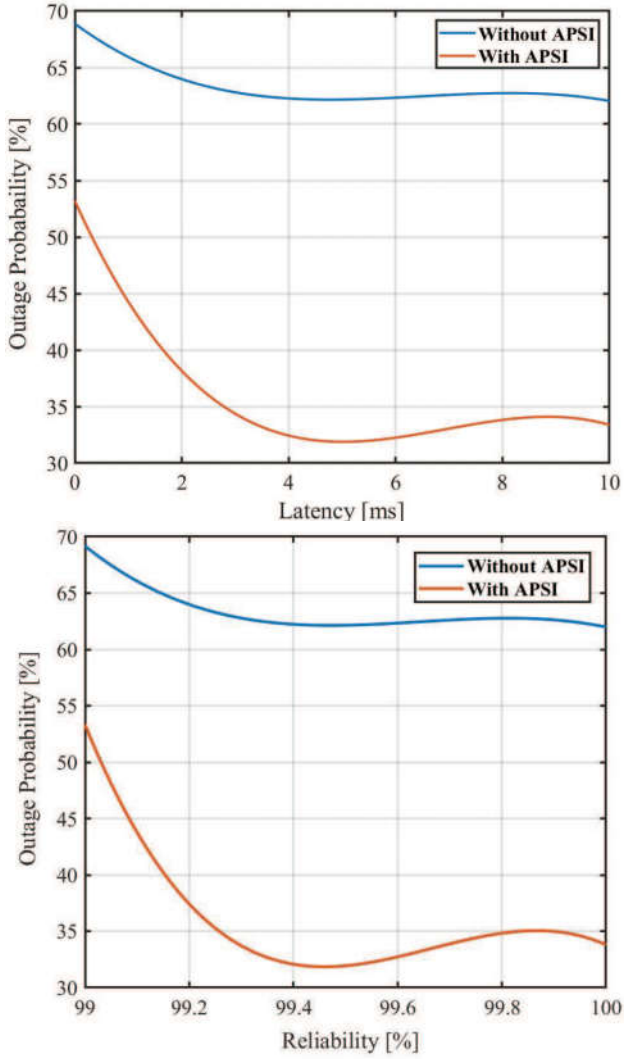
Fig. 4: Outage Probability for number of users with latency and reliability, with or without prior APSI information
