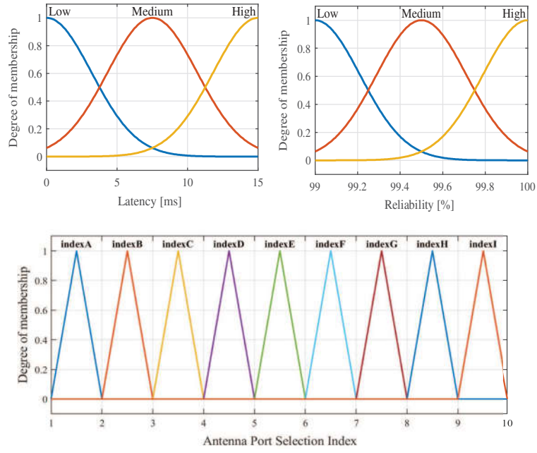
Fig. 2: Membership functions for latency, reliability and APSI in fuzzy inference system.
