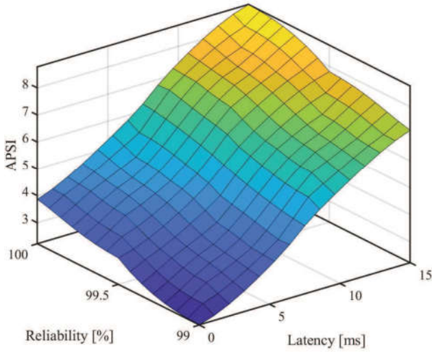
Fig. 3: APSI allocation based on latency and reliability constraints.
