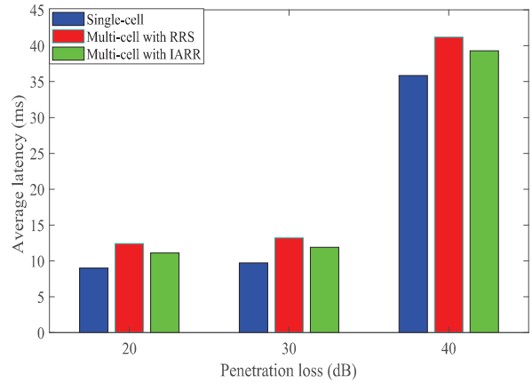
Fig. 5. Impact of penetration loss on average latency
