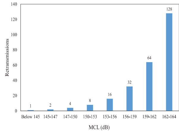
Fig. 2. Coverage classes with number of retransmissions.
