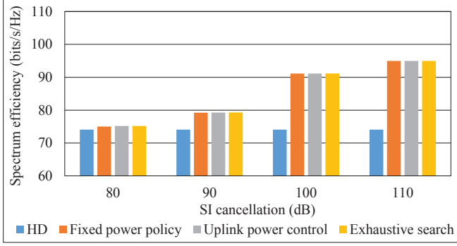
Fig. 5: Spectrum efficiency comparison for HD and FD system with asymmetric traffic at different SI cancellation level.
