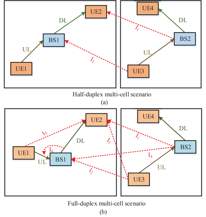
Fig. 1: Multi-cell interference scenario, where interference is considered only at BS1
