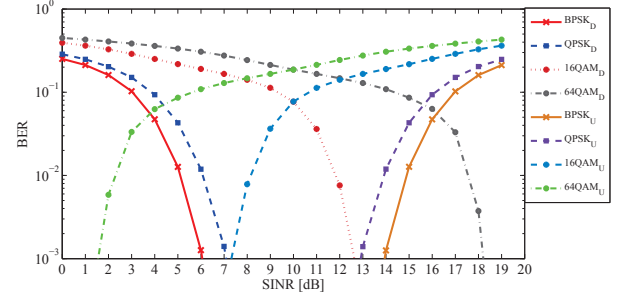
Fig. 5. BER performance of full-duplex transmission
