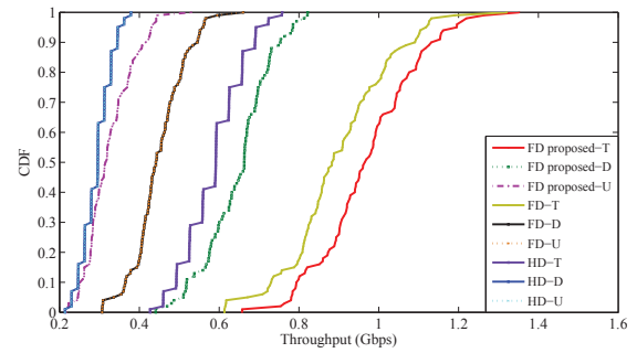
Fig. 8. Throughput performance in multiuser scenario
