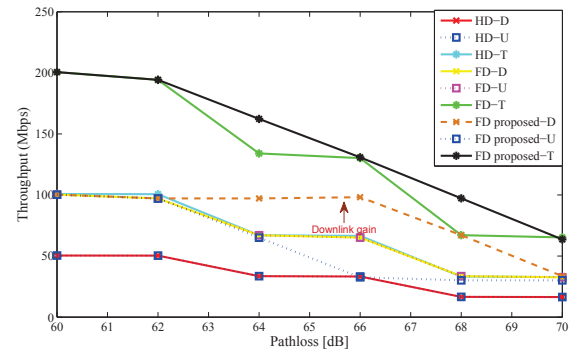
Fig. 6. Throughput performance comparison
