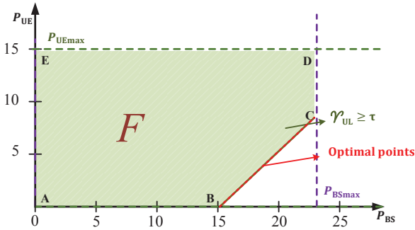
Fig. 3. Feasible region 'F': g_o=70\text{dB} , \mathcal{T}=5\text{dB} , SI_{BS}=90\text{dB} and SI_{UE}=70\text{dB}
