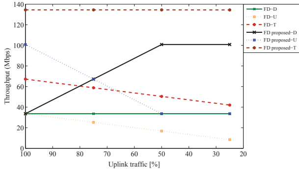
Fig. 7. Throughput comparison in asymmetric traffic
