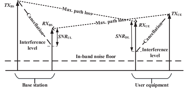
Fig. 1. Power level in full-duplex link budget
