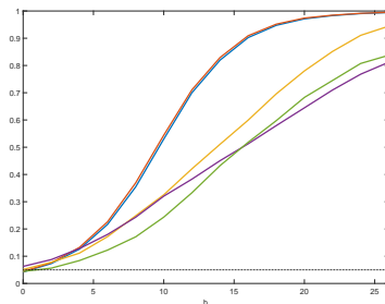
(h) \tau = 0.5 , DGP3 - Uncond. Hetero.
