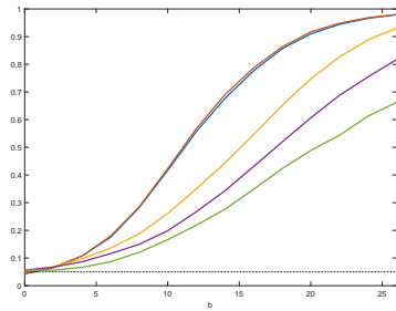
(g) \tau = 0.2 , DGP3 - Uncond. Hetero.
