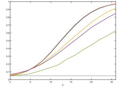
(c) \tau = 0.8 , DGP1 - AR errors
