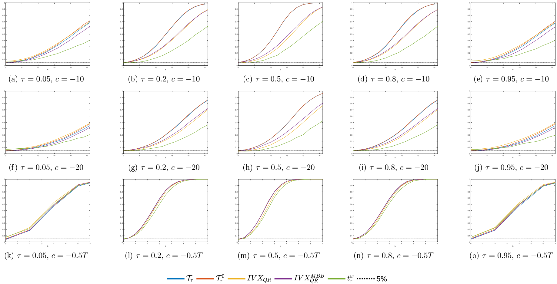
Figure D.2 (Cont.): Finite sample local power of predictability tests for T = 750 . DGP1 (homoskedastic and serially uncorrelated innovations): y_t = \beta_\tau x_{t-1} + u_{t\tau} , x_t = \rho x_{t-1} + v_t , \rho = 1 + c/T , \beta_\tau = b_\tau/T (except for c = -0.5T where \beta_\tau = b_\tau/\sqrt{T} ), b_\tau = \{0, 1, \dots, 26\} , and (u_t, v_t)' \sim i.i.d. N(\mathbf{0}, \Sigma) , with \Sigma = \begin{bmatrix} 1 & -0.95 \\ -0.95 & 1 \end{bmatrix} .
