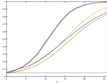
(b) \tau = 0.5 , DGP1 - AR errors
