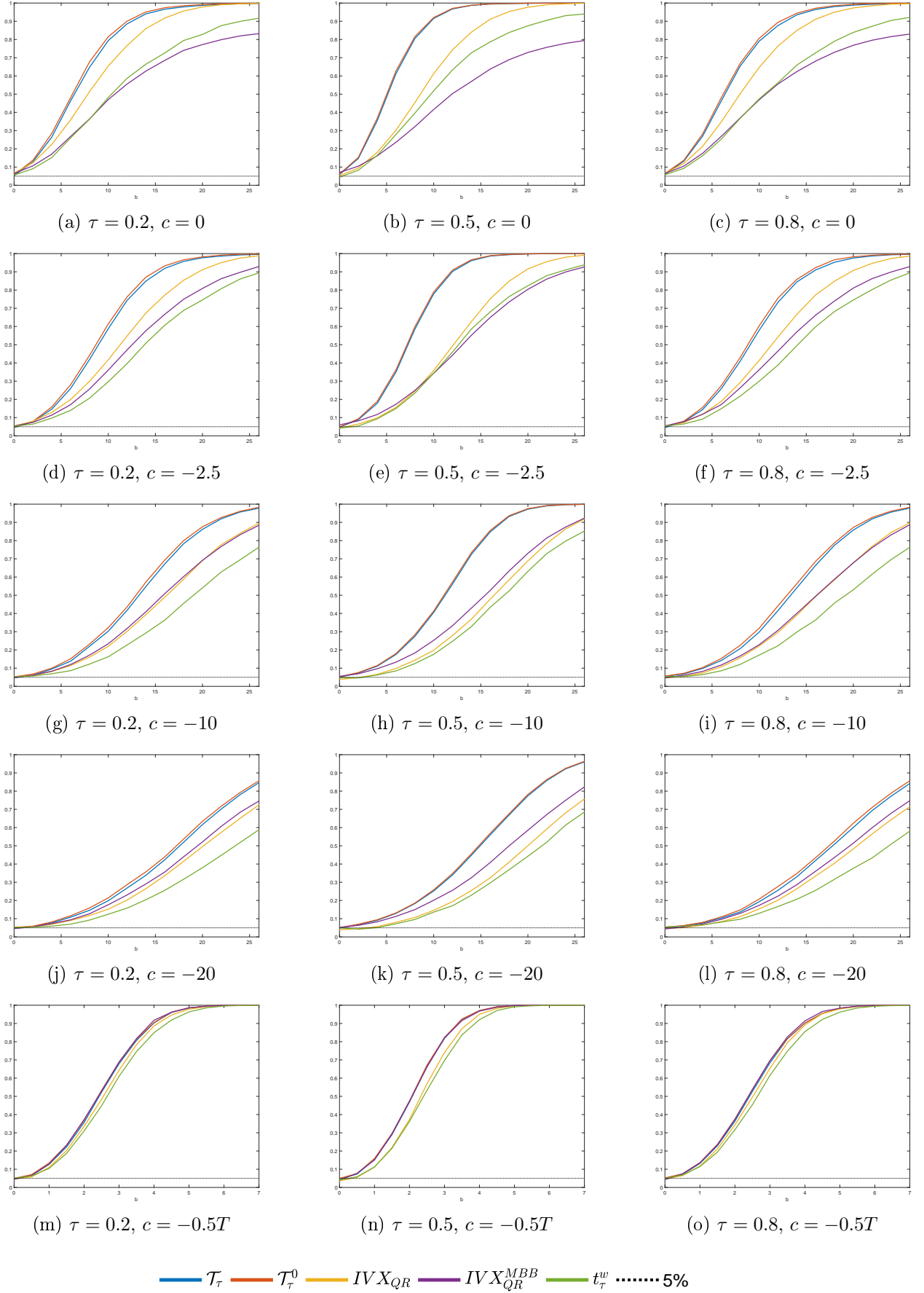
Figure 1: Finite sample local power of predictability tests for T = 250 . DGP1 (homoskedastic and serially uncorrelated innovations): y_t = \beta_\tau x_{t-1} + u_{t\tau} , x_t = \rho x_{t-1} + v_t , \rho = 1 + c/T , \beta_\tau = b_\tau/T (except for c = -0.5T where \beta_\tau = b_\tau/\sqrt{T} ), b_\tau = \{0, 1, \dots, 26\} , and (u_t, v_t)' \sim i.i.d. N(\mathbf{0}, \Sigma) , with \Sigma = \begin{bmatrix} 1 & -0.95 \\ -0.95 & 1 \end{bmatrix} .
