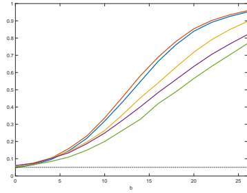
(a) \tau = 0.2 , DGP1 - AR errors
