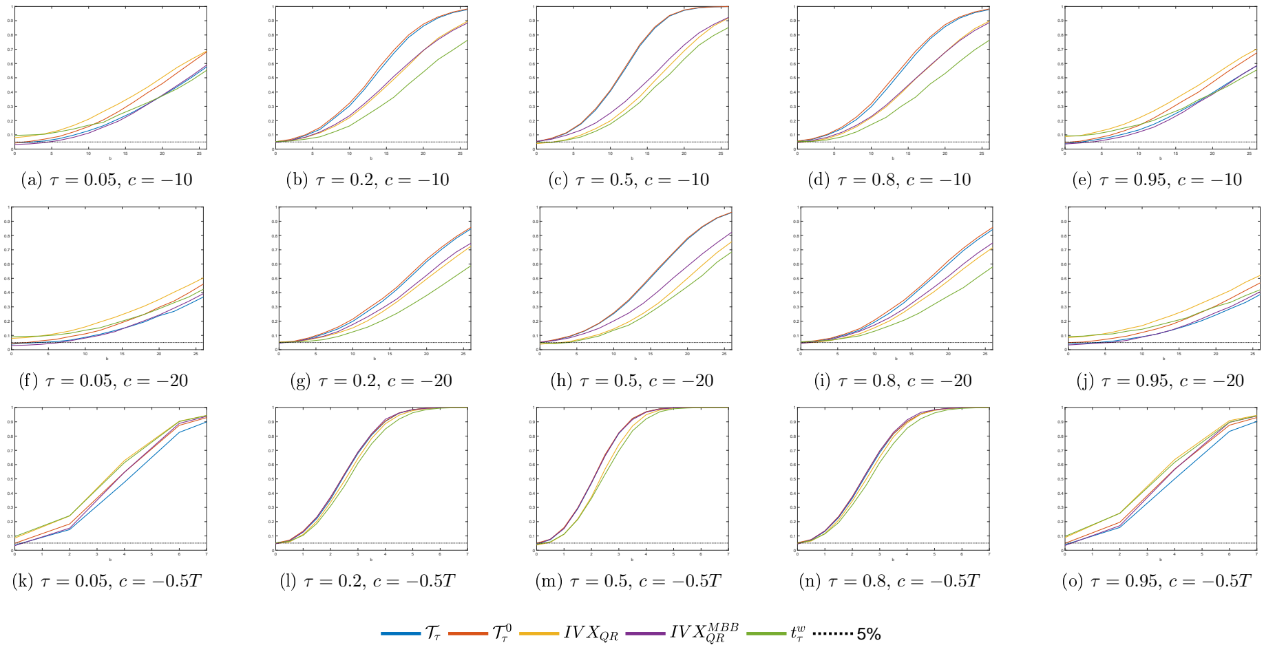
Figure D.1 (Cont.): Finite sample local power of predictability tests for T = 250 . DGP1 (homoskedastic and serially uncorrelated innovations): y_t = \beta_\tau x_{t-1} + u_{t\tau} , x_t = \rho x_{t-1} + v_t , \rho = 1 + c/T , \beta_\tau = b_\tau/T (except for c = -0.5T where \beta_\tau = b_\tau/\sqrt{T} ), b_\tau = \{0, 1, \dots, 26\} , and (u_t, v_t)' \sim i.i.d. N(\mathbf{0}, \Sigma) , with \Sigma = \begin{bmatrix} 1 & -0.95 \\ -0.95 & 1 \end{bmatrix} .
