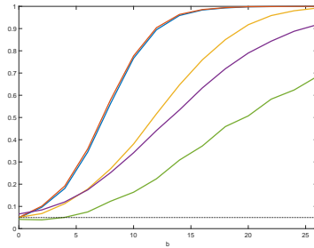
(e) \tau = 0.5 , DGP2a - GARCH(1,1)
