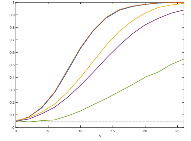
(f) \tau = 0.8 , DGP2a - GARCH(1,1)
