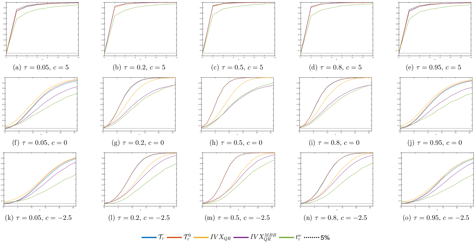
Figure D.2: Finite sample local power of predictability tests for T = 750 . DGP1 (homoskedastic and serially uncorrelated innovations): y_t = \beta_\tau x_{t-1} + u_{t\tau} , x_t = \rho x_{t-1} + v_t , \rho = 1 + c/T , \beta_\tau = b_\tau/T (except for c = -0.5T where \beta_\tau = b_\tau/\sqrt{T} ), b_\tau = \{0, 1, \dots, 26\} , and (u_t, \varepsilon_t)' \sim i.i.d. N(\mathbf{0}, \Sigma) , with \Sigma = \begin{bmatrix} 1 & -0.95 \\ -0.95 & 1 \end{bmatrix} .
