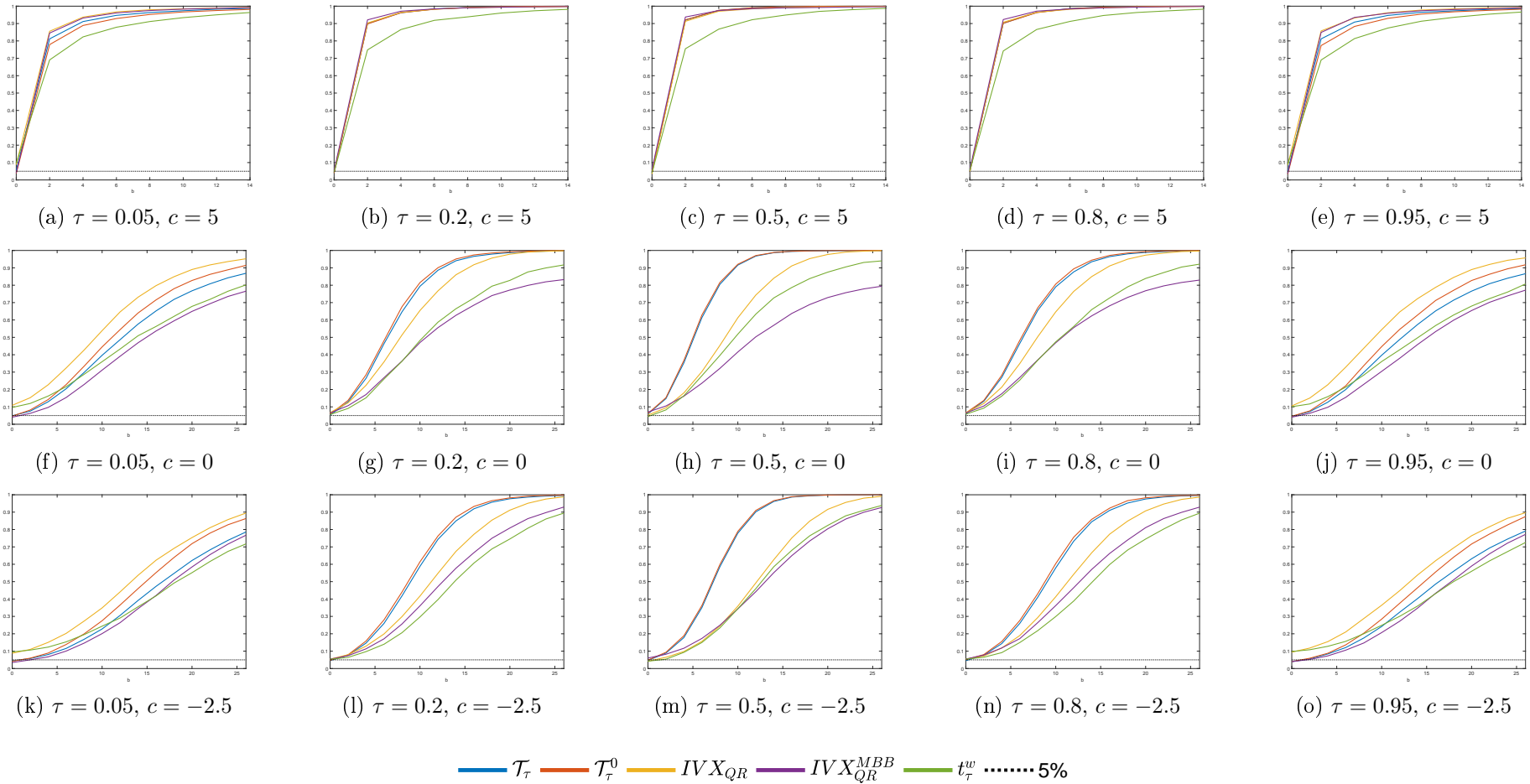
Figure D.1: Finite sample local power of predictability tests for T = 250 . DGP1 (homoskedastic and serially uncorrelated innovations): y_t = \beta_\tau x_{t-1} + u_{t\tau} , x_t = \rho x_{t-1} + v_t , \rho = 1 + c/T , \beta_\tau = b_\tau/T (except for c = -0.5T where \beta_\tau = b_\tau/\sqrt{T} ), b_\tau = \{0, 1, \dots, 26\} , and (u_t, v_t)' \sim i.i.d. N(\mathbf{0}, \Sigma) , with \Sigma = \begin{bmatrix} 1 & -0.95 \\ -0.95 & 1 \end{bmatrix} .
