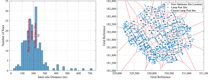
Fig. 5: ISD distribution built to 200 m (45 new sites).
