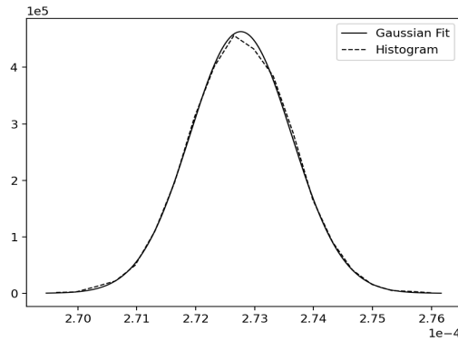
Figure 3: Histogram of the deflection data, w_1 , from time T and distribution fitted to the data.
