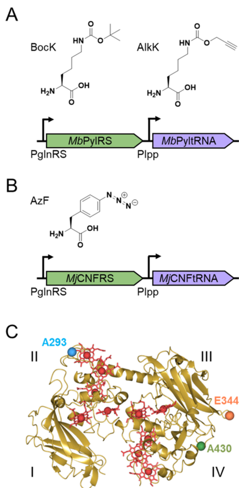
Figure 2. ncAA insertion systems used in our studies. (A) MbPylRS / PyltRNA CUA pair incorporates N ε -Boc-L-lysine (BocK) and N ε -(4-pentynyloxycabonyl)-L-lysine (AlkK). (B) MjCNFRS / tRNA pair incorporates p -azido-L-phenylalanine (AzF). (C) Crystal structure of wtMtrC (PDB ID: 4LM8) indicating domains I–IV, the 10 covalently attached c -hemes (red), and the locations of residues selected for replacement by ncAA (A293, E344, A430).
