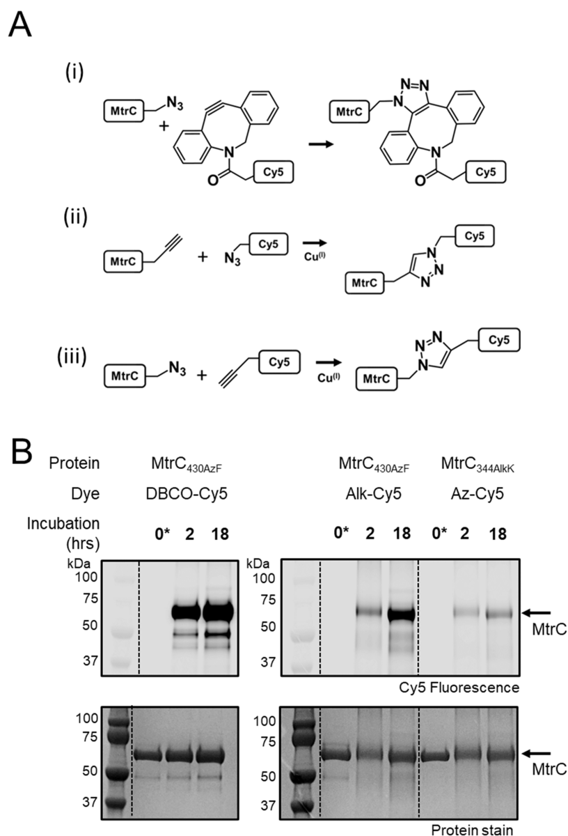
Figure 6. Introduction of fluorescent probes to nAA-containing MtrC proteins using bioorthogonal chemistry. (A) Reactions explored in this study. (i) Strain-promoted azide–alkyne cycloaddition with dibenzocyclooctyne sulfo-cyanine 5 (DBCO-Cy5). (ii), (iii) Copper-catalyzed azide–alkyne cycloaddition with functionalized Cy5 dyes. (B) SDS-PAGE gel images for samples of nAA-containing MtrC proteins incubated with functionalized Cy5 dyes, as indicated. Upper panel: Cy5 dye visualized by fluorescence emission (excitation at 635 nm). Lower panel: proteins visualized by Coomassie stain. Arrows indicate the expected migration of MtrC proteins.
