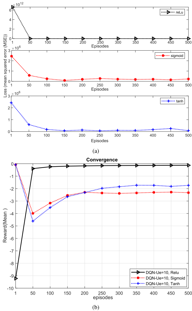
Fig. 7. Overview of the proposed framework for the sum-rate maximization problem. Sub-figure (a) DRL loss vs the number of episodes: A comparison between DRL loss and training episodes for different activation functions (ReLU, TanH, Sigmoid). Sub-figure (b) shows Rewards vs activation functions: A comparison between achieved rewards and episodes for different activation functions (ReLU, TanH, Sigmoid) of DRL algorithm.
