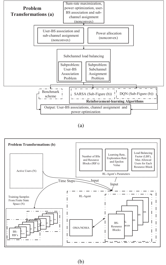
Fig. 2. Overview of the proposed framework for the sum-rate maximization problem. Sub-figure (a) is an optimization problem breakdown to show where RL algorithms are applied and Sub-figure (b) shows problem transformations for the users and BSs as system states and the brain of reinforcement learning agents, respectively.
