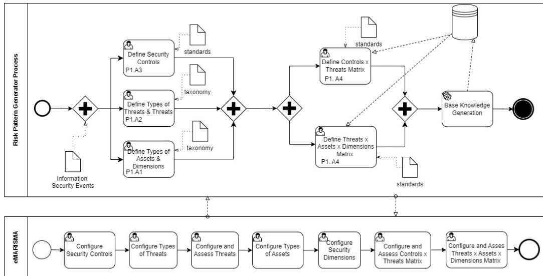
Figure 8: Risk Pattern Generator Process
