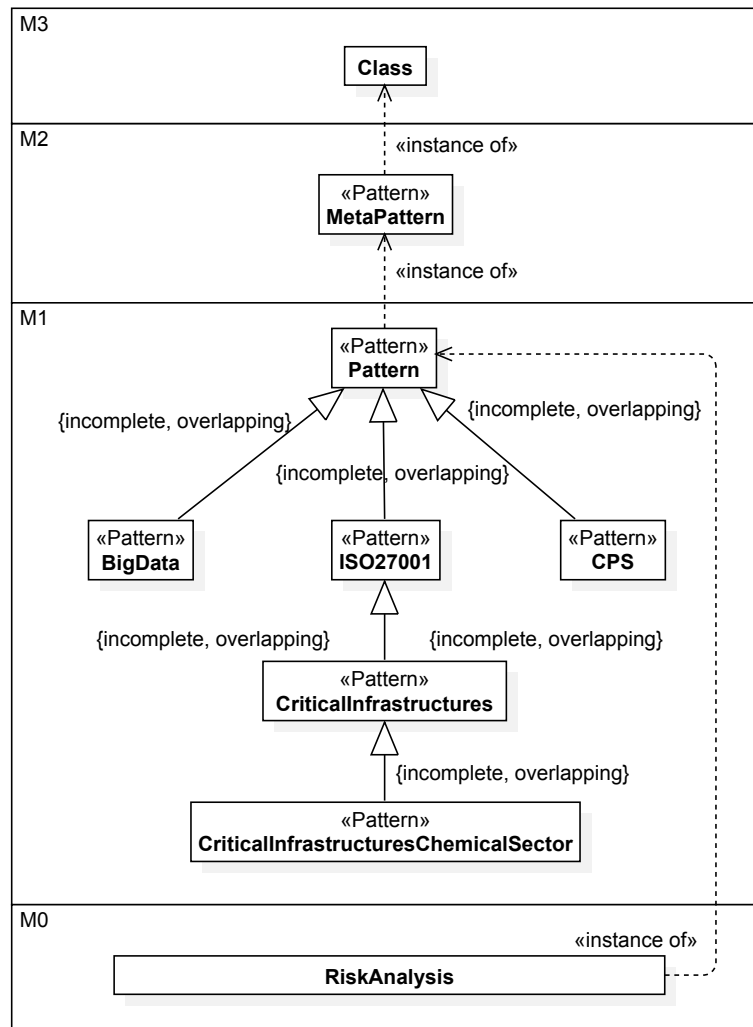
Figure 2: Pattern inheritance and instantiation
