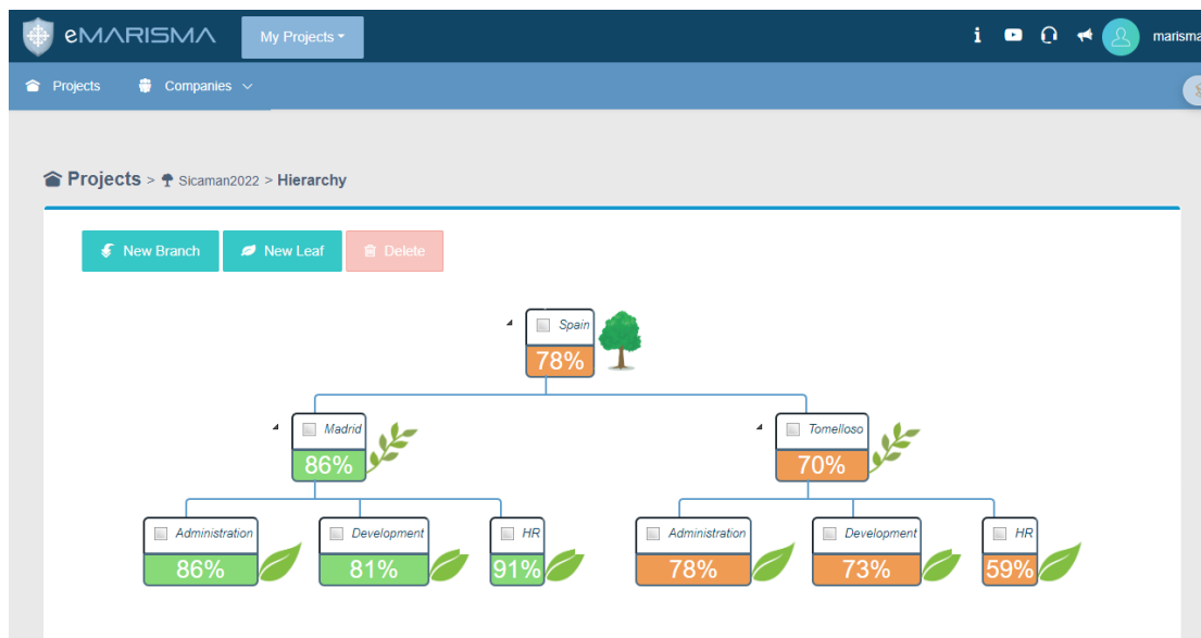
Figure 11: Hierarchy tree in eMARISMA
