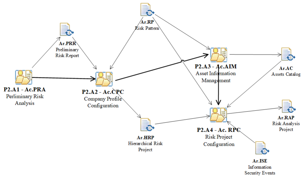
Figure 6: Diagram of activities, inputs and outputs. RAMG process
