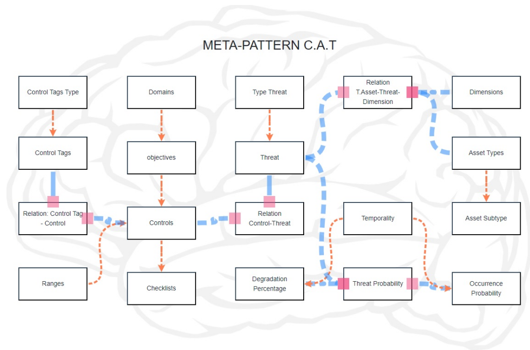
Figure 9: Meta-Pattern structure guide in eMARISMA
