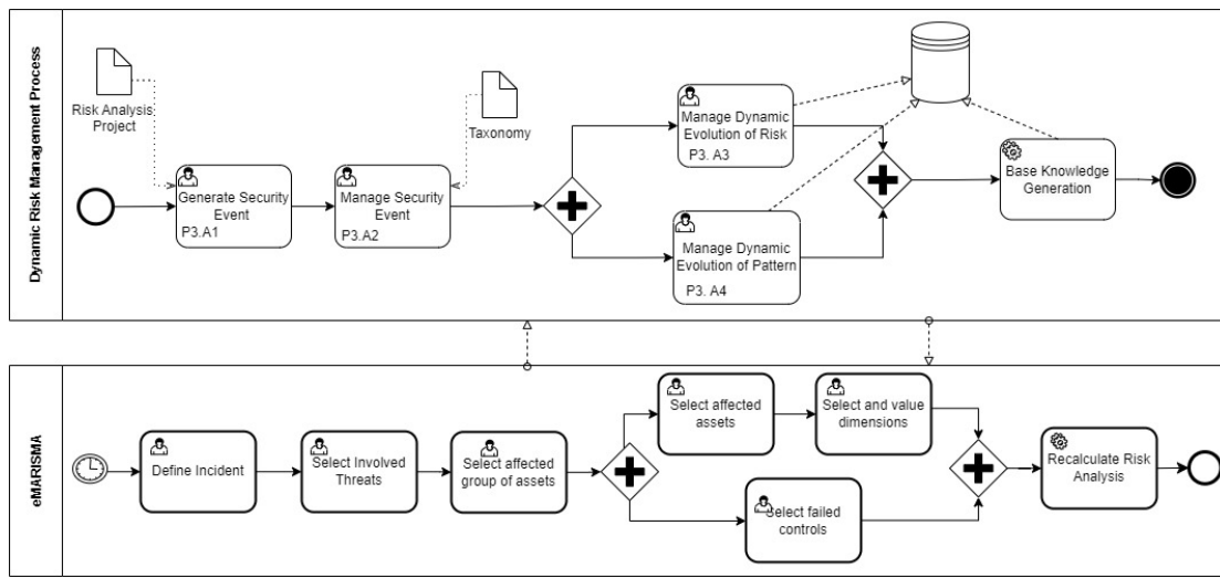
Figure 13: Dynamic Risk Management Process
