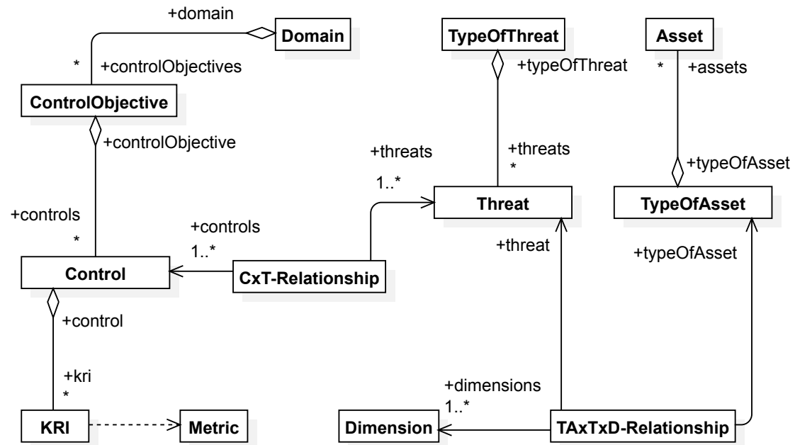
Figure 3: Meta-pattern CAT (detailed view)
