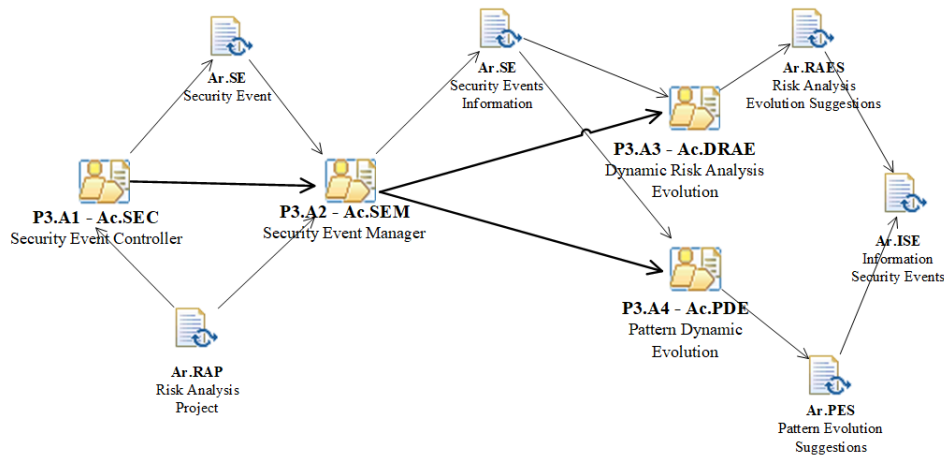
Figure 7: Diagram of activities, inputs and outputs. DRM process
