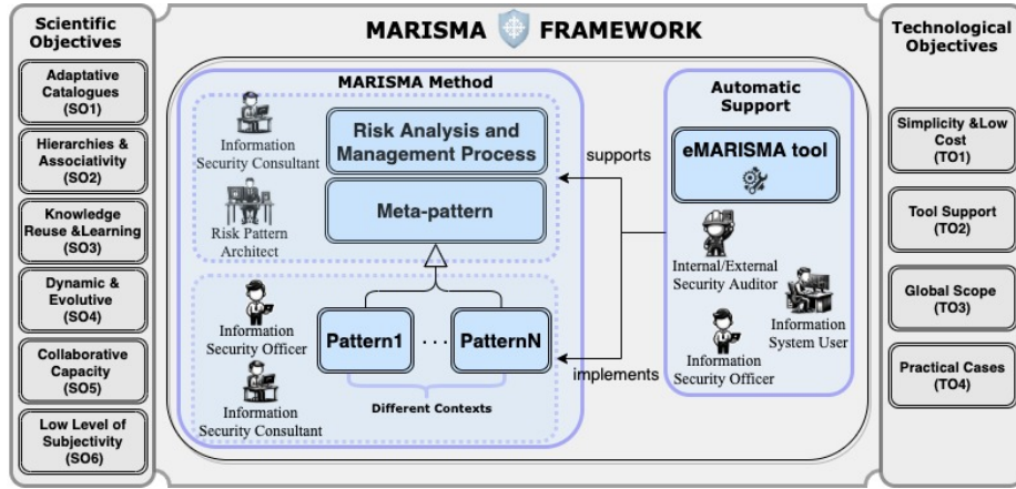
Figure 1: Architecture of our MARISMA framework
