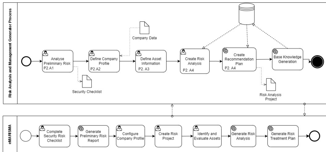
Figure 10: Risk Analysis and Management Generator Process
