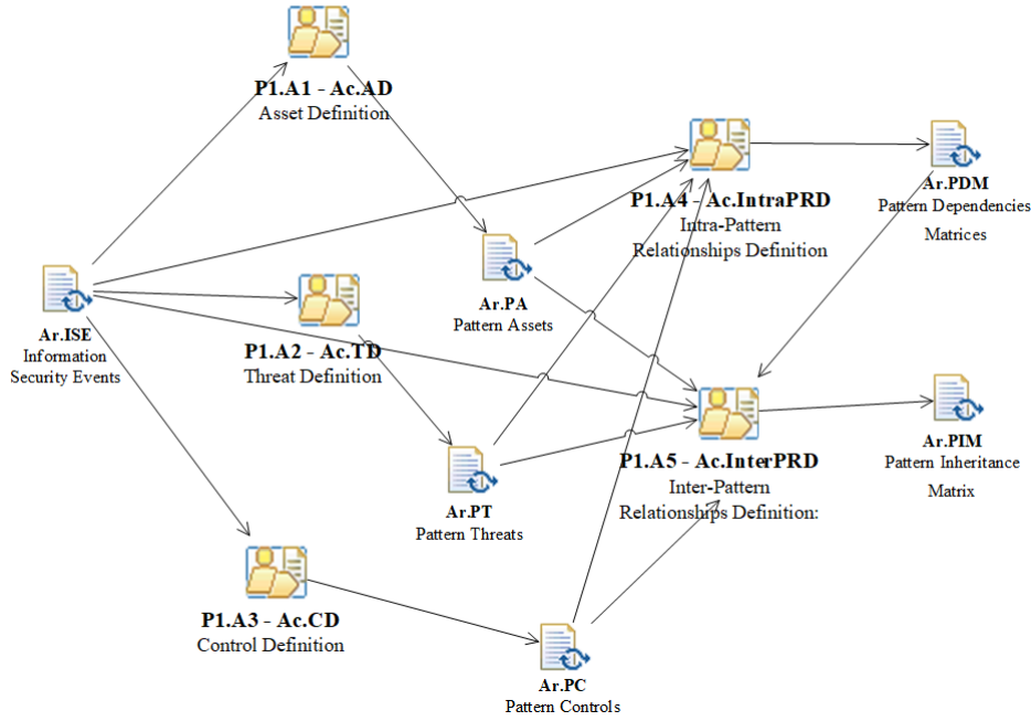
Figure 5: Diagram of activities, inputs and outputs. RPG process
