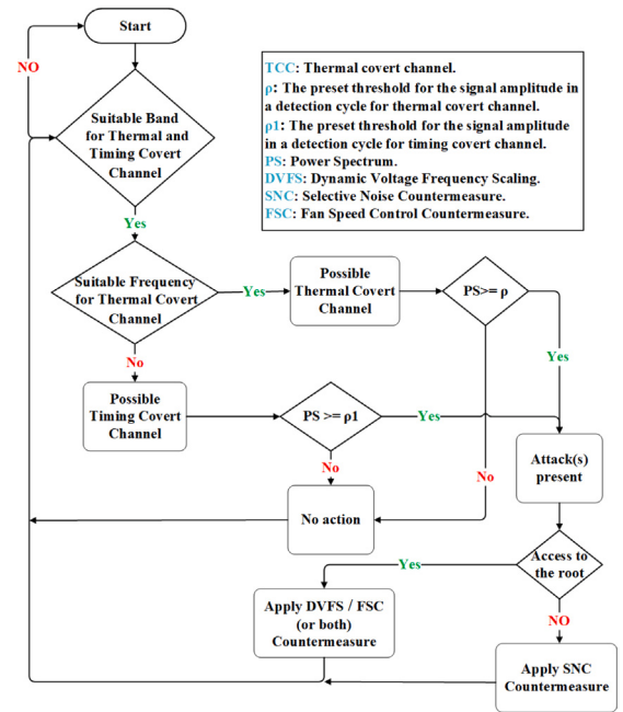
Fig. 2. Diagram of process of detection and defence of Thermal and Timing Covert Channel Attacks in double covert channels (process1).
