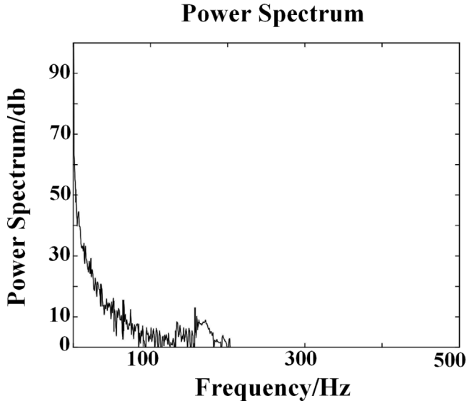
Fig. 7. Double covert channel with DVF and fan speed countermeasure.
