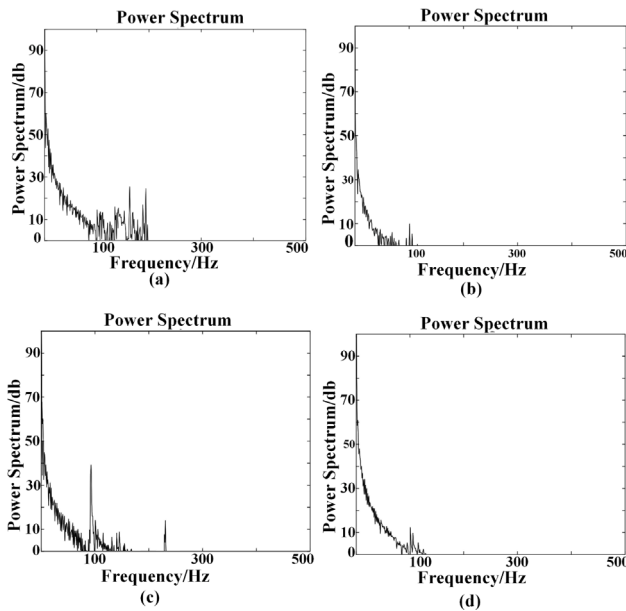
Fig. 5. Thermal and Timing covert channel attacks are using a single channel. (a) Multi attacks without countermeasure, (b) Multi attacks with DVFS countermeasure, (c) Multi attacks with selective noise countermeasure, (d) Multi attacks with Fan speed control counter.
