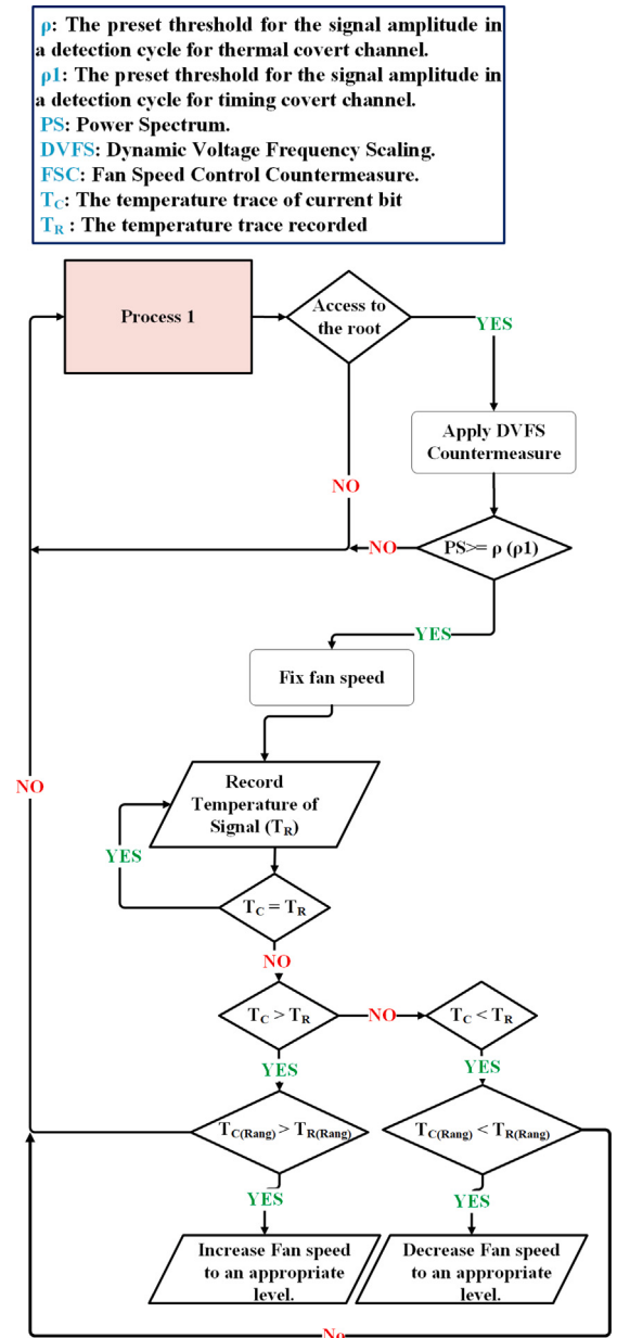
Fig. 6. Diagram of the process combined defence strategy in multi-covert channels.
