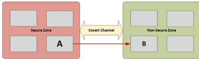
Fig. 1. Covert Channel communication in an eight multicore system. The arrow from core A to core B indicates that the data/information flows from core A to core B.
