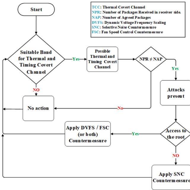
Fig. 4. Diagram of process of detection and defence of Thermal and Timing Covert Channel Attacks in single covert channels (process1).
