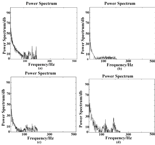
Fig. 3. System behaviour with double covert channels, (a) system without countermeasure, (b) system with DVFS countermeasure, (c) system with Selective Noise countermeasure and (d) system with Fan Speed Control countermeasure.
