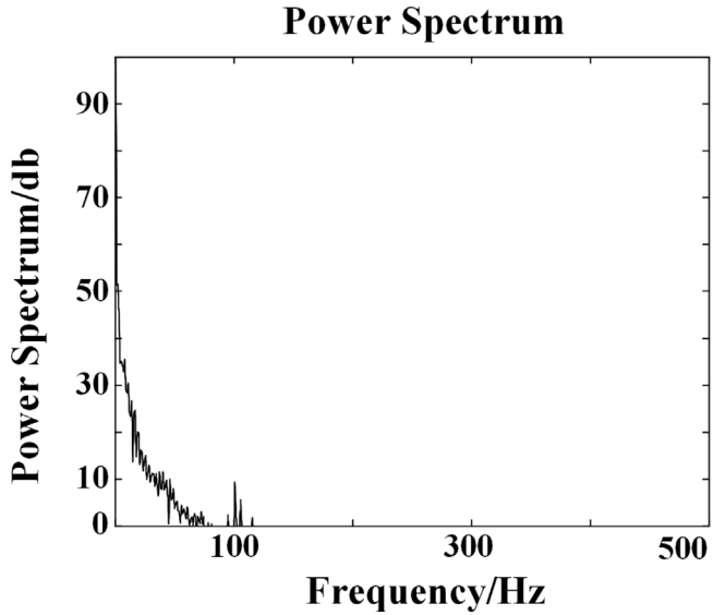
Fig. 8. Single covert channel with DVF and fan speed countermeasure.
