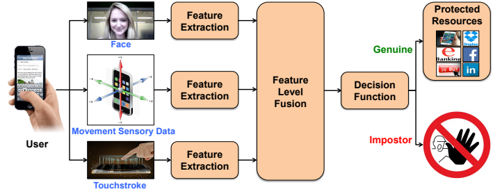
Fig. 1. Proposed smartphone user authentication framework.
