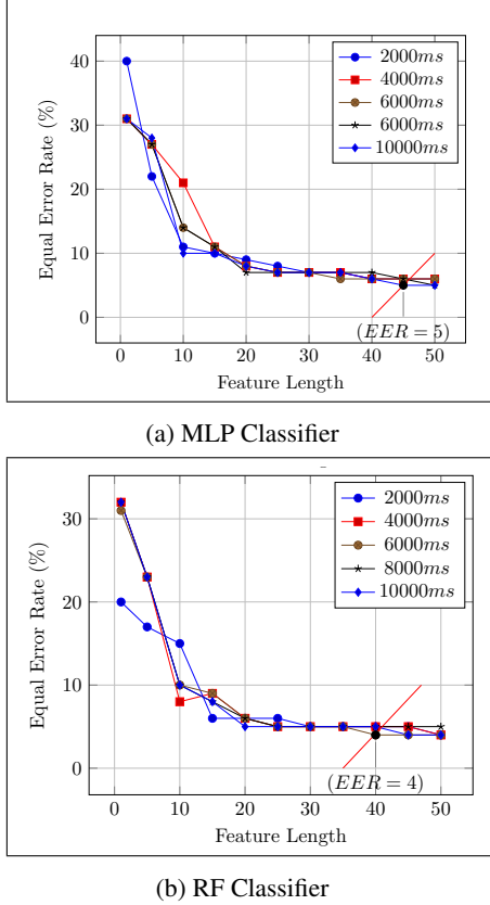
Figure 6: Results in terms of EER for different feature lengths (from selected features).
