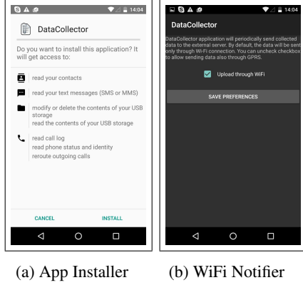
Figure 3: Screen shots of our DataCollector app: Figure 3a shows the application installer and the Figure 3b shows the connectivity manager.
