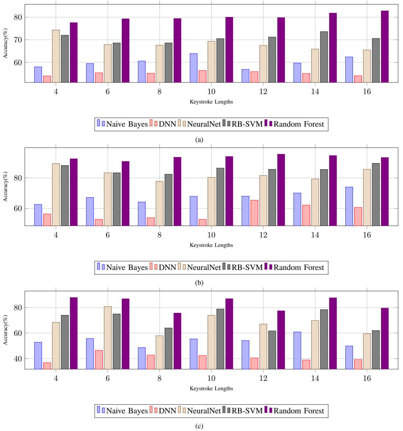
Fig. 2: Bar graphs for (a) gender, (b) operating-hand, and (c) age estimation for different keystroke lengths obtained from all the classifiers
