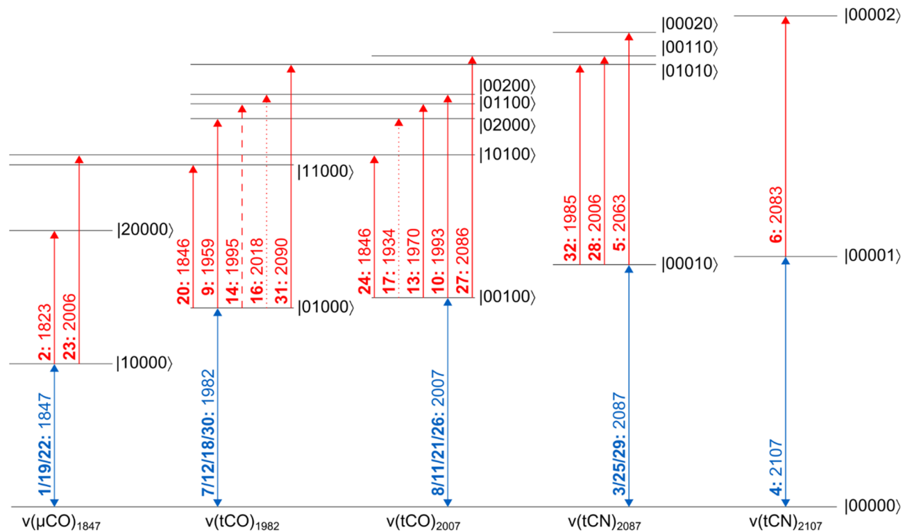
Fig. 3 Energy level scheme illustrating the vibrational transitions probed in this study. All energy eigenstates are labelled as |abcde>, where each entry refers to the number of vibrational quanta in each one of the five vibrational modes (listed by increasing frequency). Dipole-forbidden transitions are shown as dotted lines. A weakly resolved transition is depicted as a dashed line. Signals are labelled as bold numbers according to the main text. All transitions energies, given in units of cm -1 , correspond to the probe frequencies of the indicated signals.
