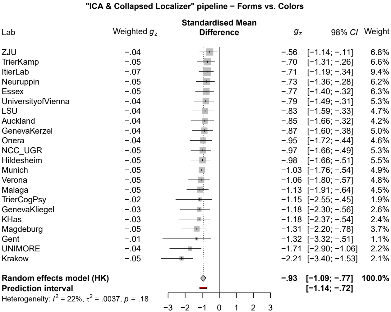
Fig. 16 – Forest plot of the meta-analysis for Difference in the “ICA & Collapsed localizer” pipeline.
