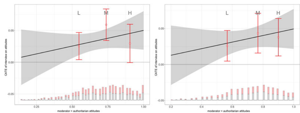
Figure 4. Conditional average treatment effects of unchallenged interview on agreement with extreme right statements, conditional on authoritarian attitudes in Australia (left) and the UK (right): 95 per cent confidence intervals.
